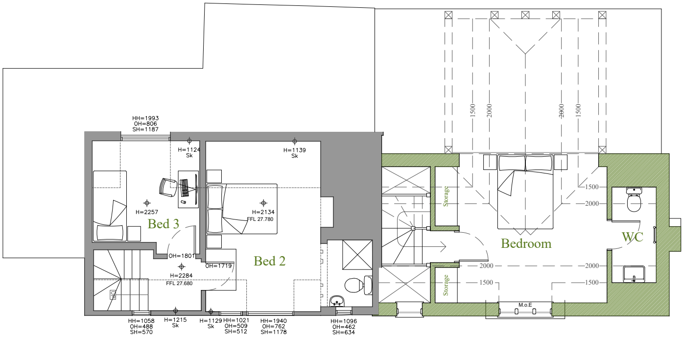
First Floor
