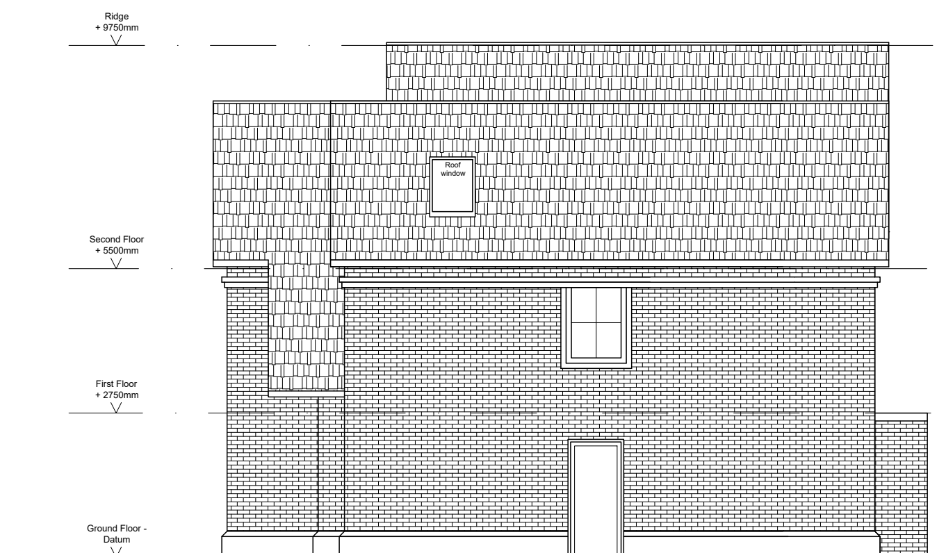
SIDE ELEVATION (PLOT 2-5)
