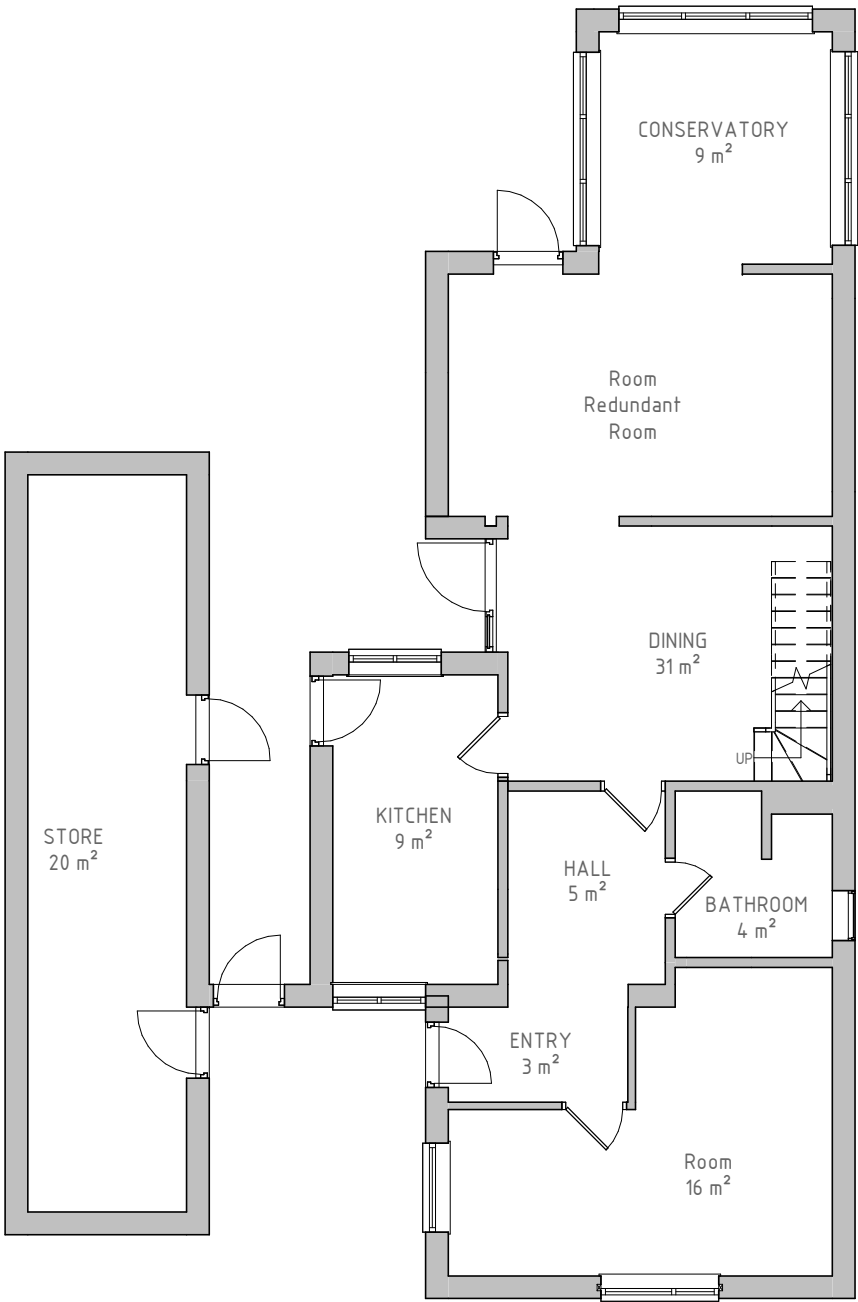
03/101 - EXISTING GROUND FLOOR PLAN 1: 100
