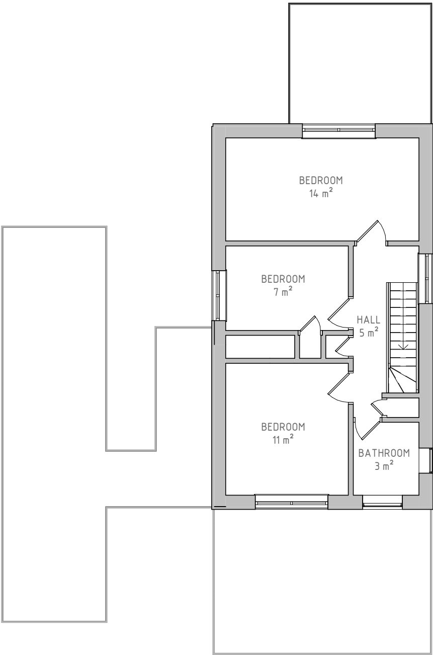
03/102 - EXISTING FIRST FLOOR PLAN 1: 100
