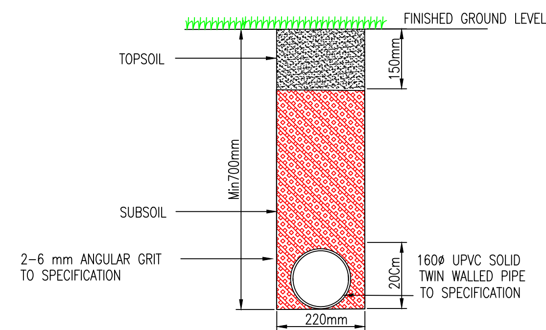
150Ø CUT-OFF/CARRIER DRAIN
