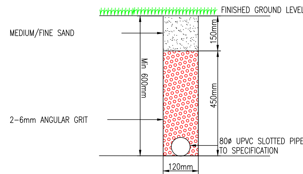
80Ø LATERAL DRAIN
