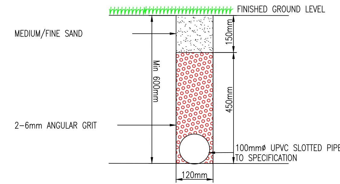
100Ø LATERAL DRAIN
