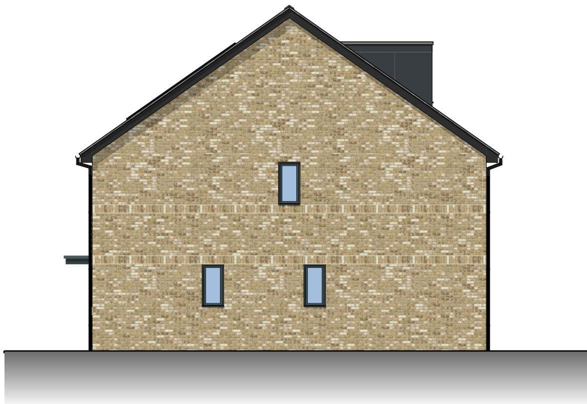
UNIT TYPE A & B - NORTH (SIDE) ELEVATION
