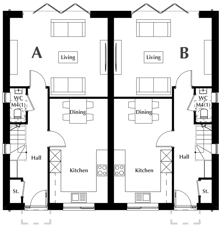
UNIT TYPE A & B - GROUND FLOOR PLAN
