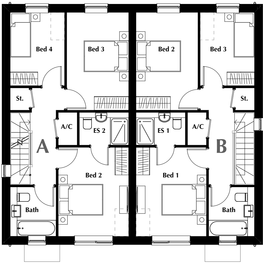
UNIT TYPE A & B - FIRST FLOOR PLAN
