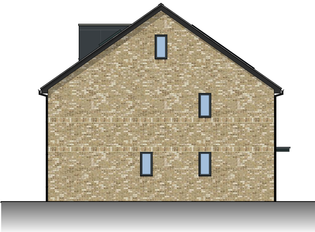
UNIT TYPE A & B - SOUTH (SIDE) ELEVATION
