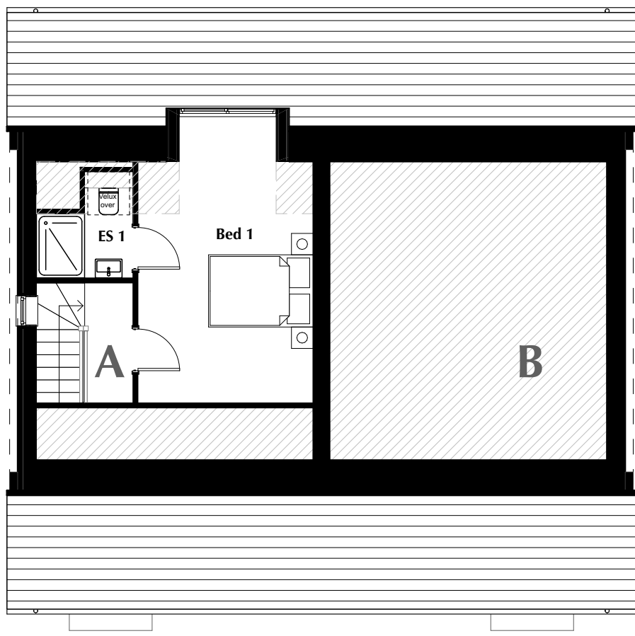
UNIT TYPE A & B - SECOND FLOOR PLAN
