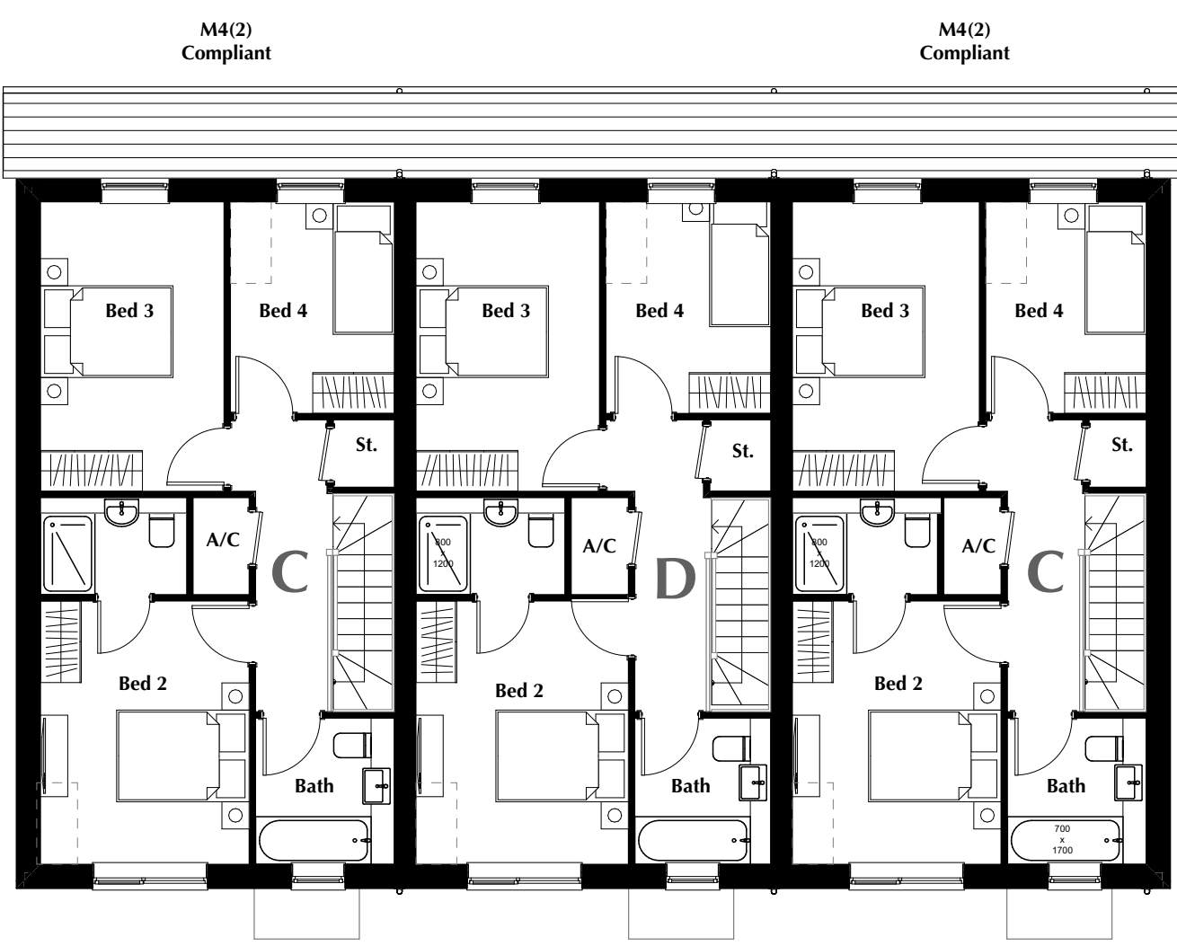
UNIT TYPE C & D - FIRST FLOOR PLAN
