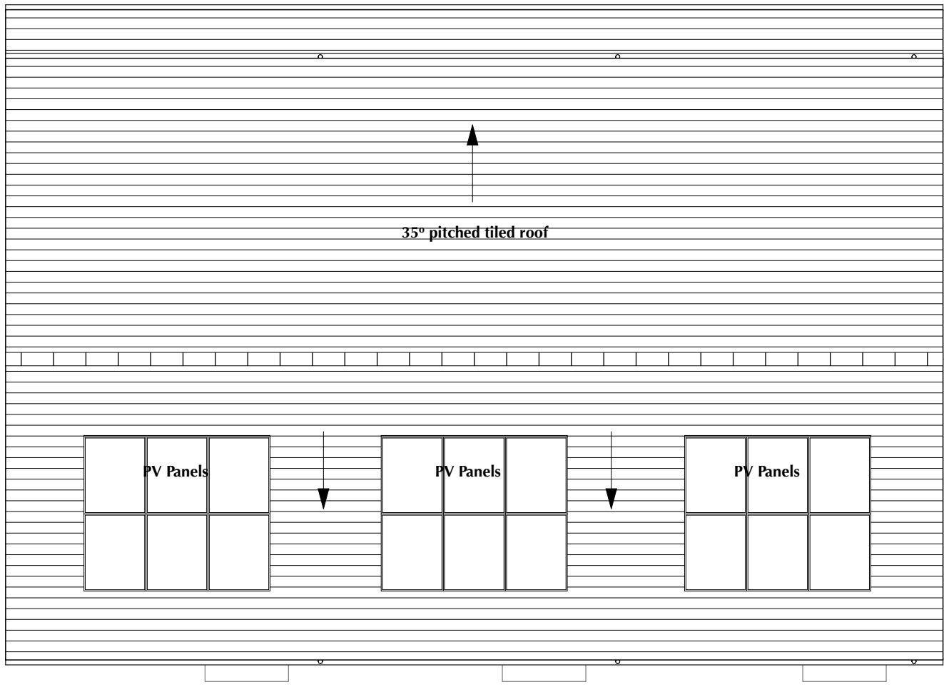
UNIT TYPE C & D - ROOF PLAN
