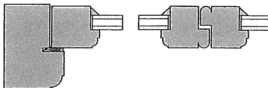
Jamb / Head Section Scale 1:2 @ A3
