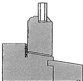
Jamb / Head Section Scale 1:2 @ A3
