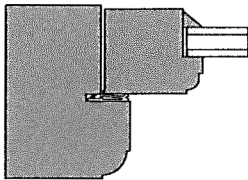
Jamb / Head Section Scale 1:2 @ A3
