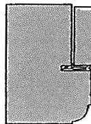
Jamb / Head Section Scale 1:2 @ A3
