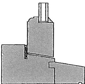
Jamb / Head Section Scale 1:2 @ A3
