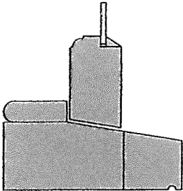
Sill Section Scale 1:2 @ A3
