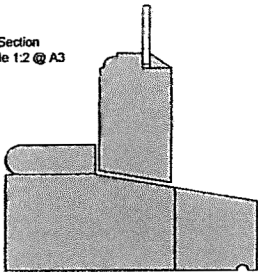
Jamb / Head Section Scale 1:2 @ A3
