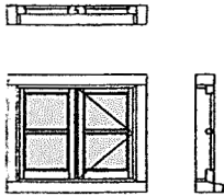
M5 - Double Rebated Casement Internal View 1:20 @ A3
