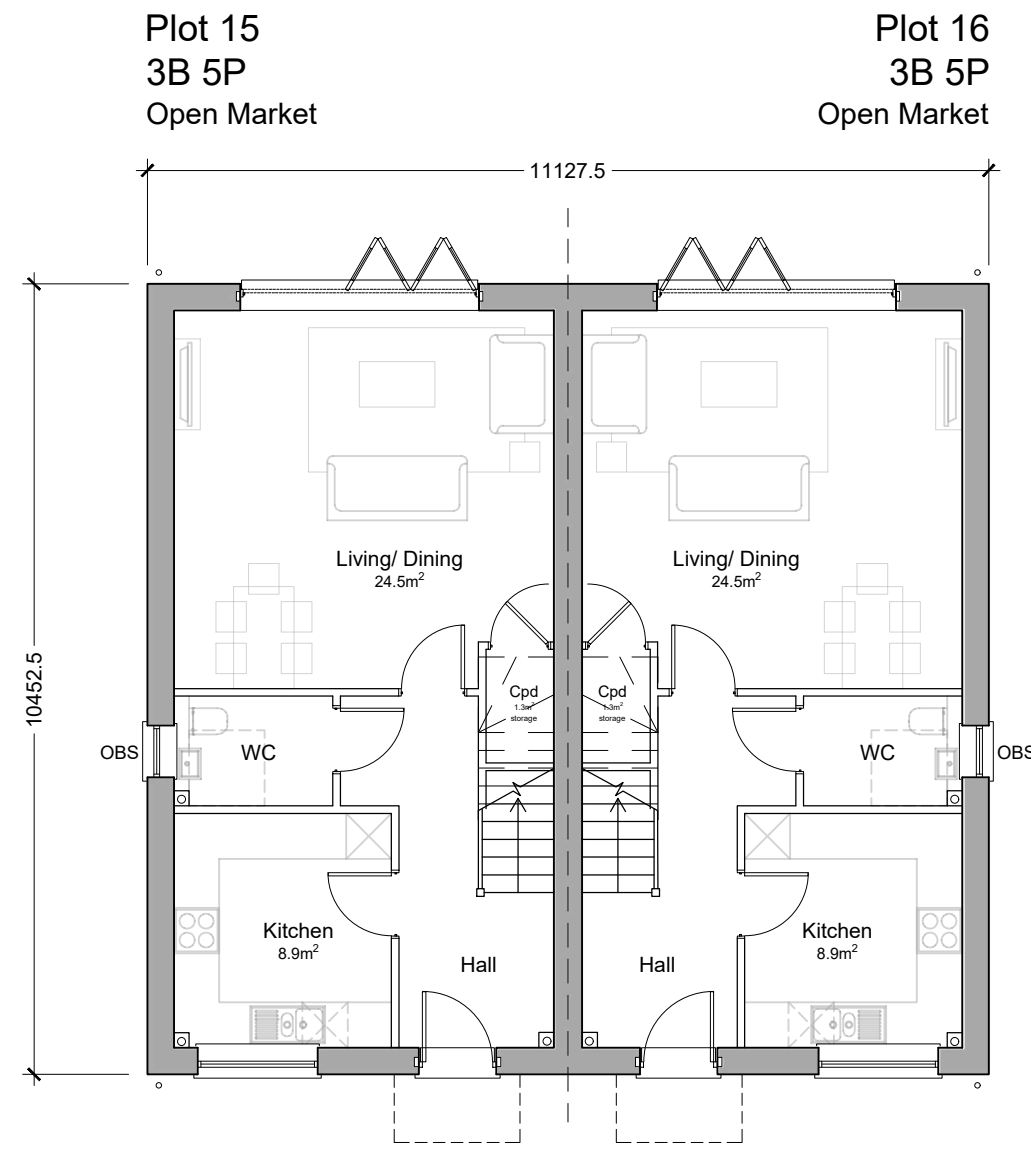
GROUND FLOOR
