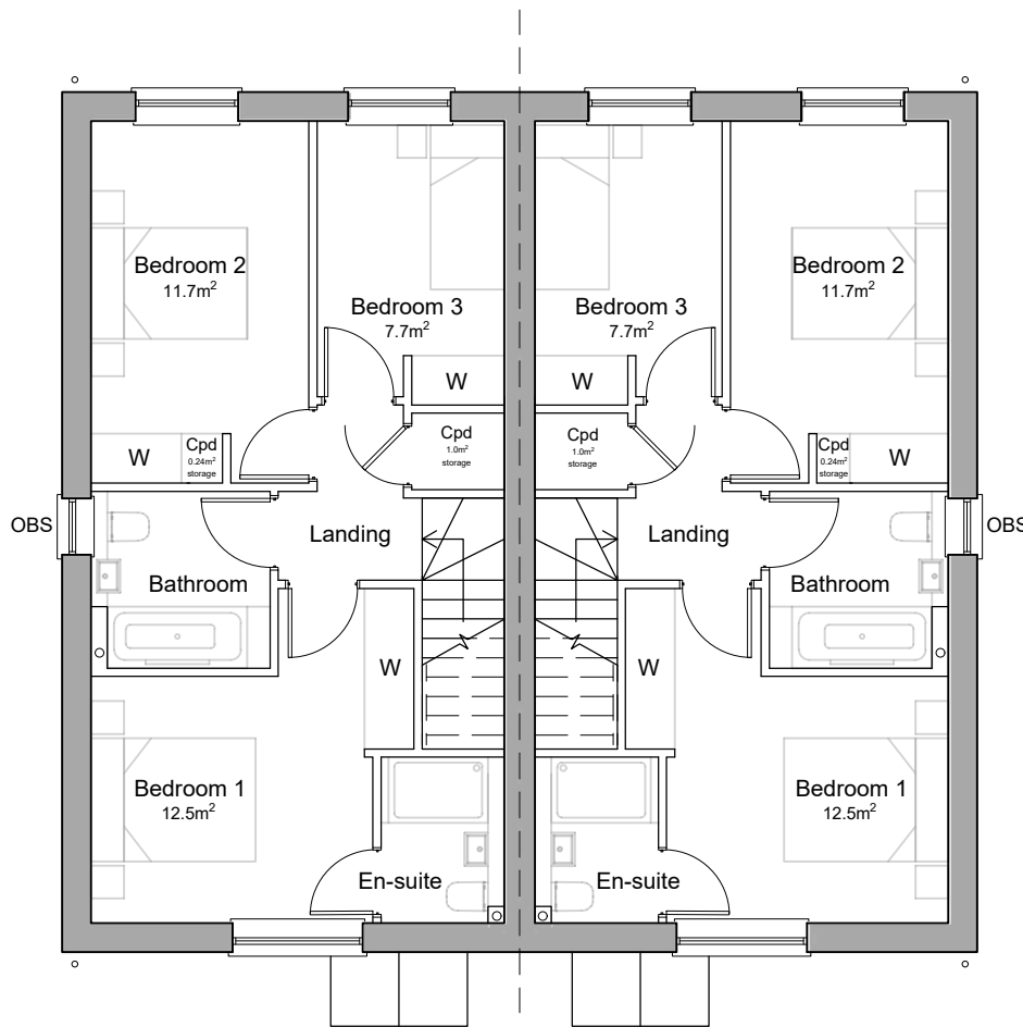
FIRST FLOOR
