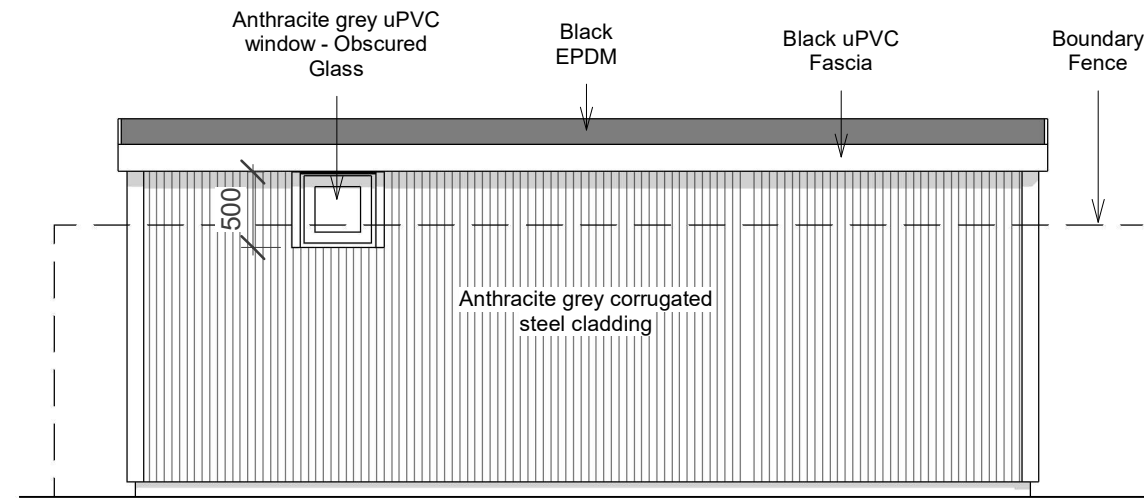
East (Rear) Elevation
