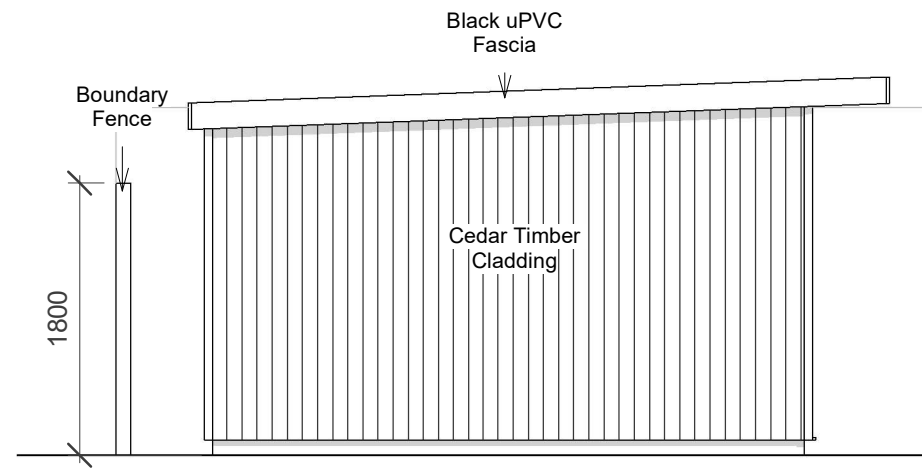
North (Left) Elevation
