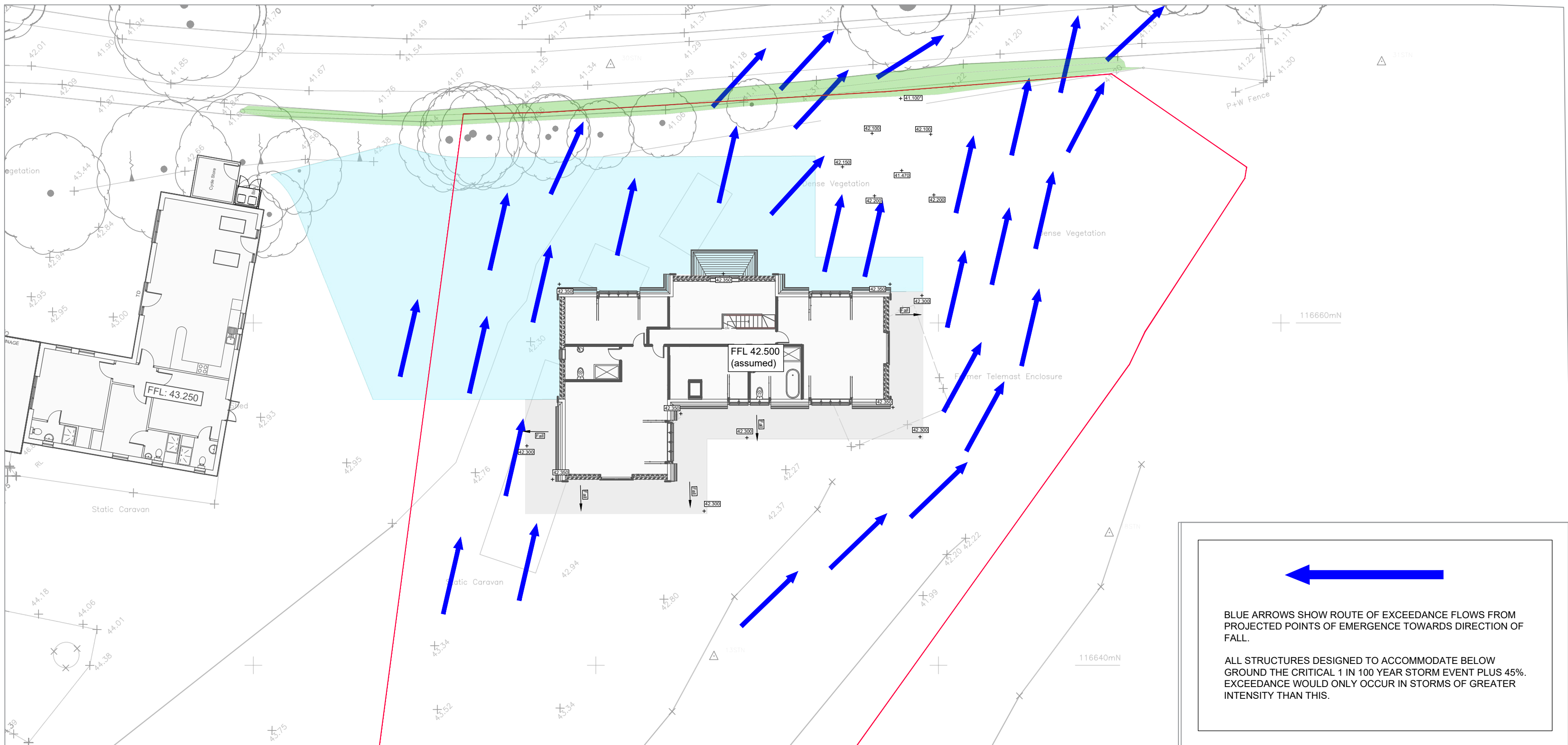
EXCEEDANCE FLOW ROUTES (scale 1:200)
