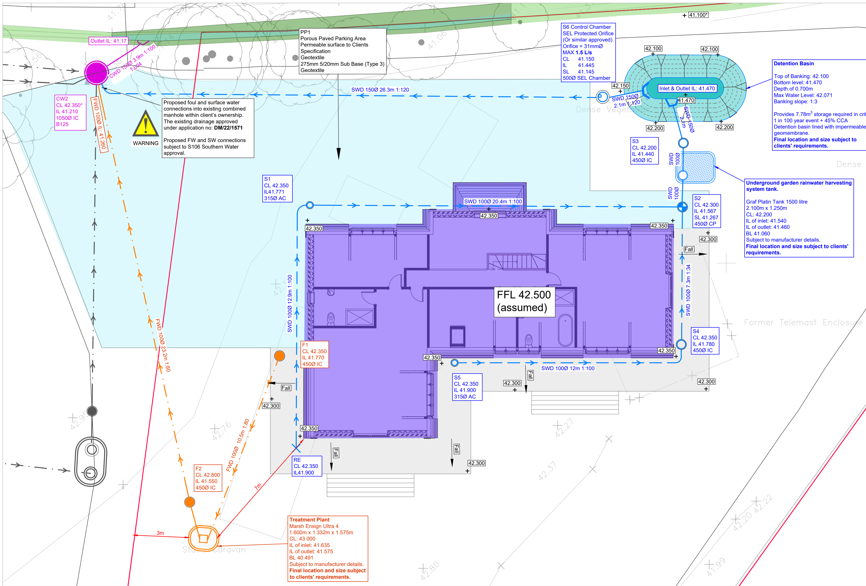
PROPOSED DRAINAGE STRATEGY (scale 1:100)
