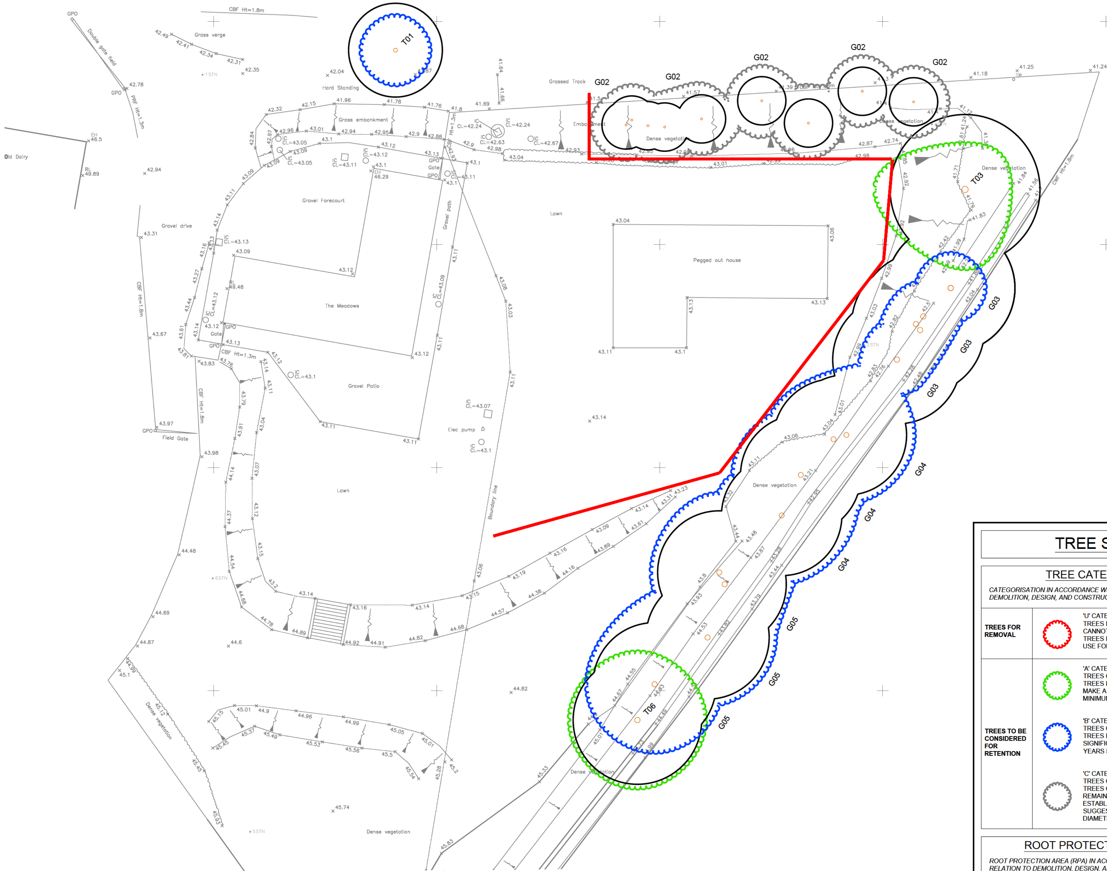
TREE PROTECTION PLAN (1:200)
