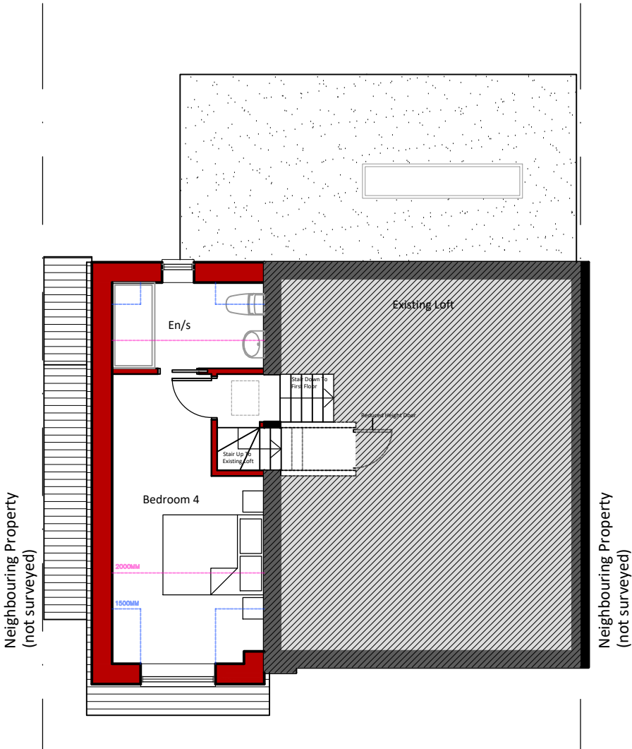
Proposed Upper First Floor Plan Scale 1:100
