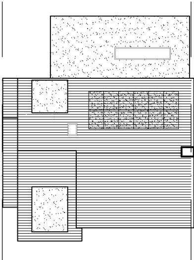
Proposed Roof Plan Scale 1:200
