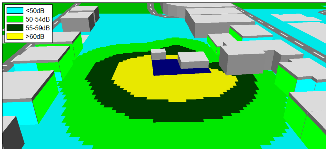
External Play Area Noise Propagation (CadnaA Noise Map)
