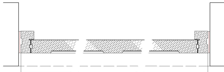
FRONT DOOR PLAN DETAIL - AS PROPOSED SCALE @ 1:5 ON AN A1 SHEET
