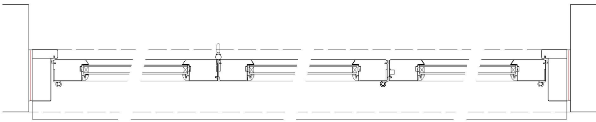
BI-FOLDING DOOR PLAN DETAIL - AS PROPOSED SCALE @ 1:5 ON AN A1 SHEET
