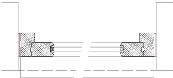
SINGLE GLAZED DOOR PLAN DETAIL - AS PROPOSED SCALE @ 1:5 ON AN A1 SHEET
