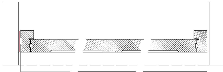
STABLE DOOR PLAN DETAIL - AS PROPOSED SCALE @ 1:5 ON AN A1 SHEET
