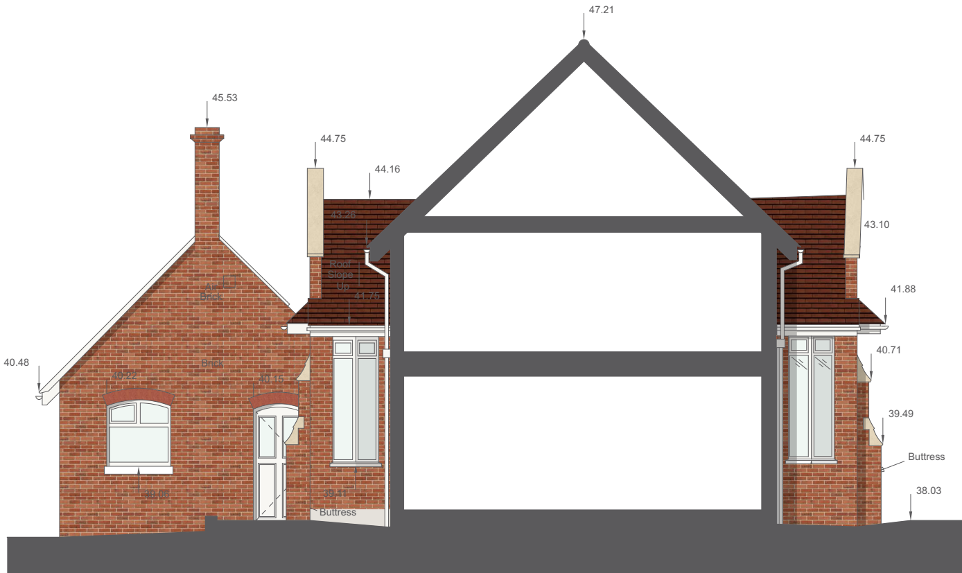
03 - PROPOSED SECTION 3
