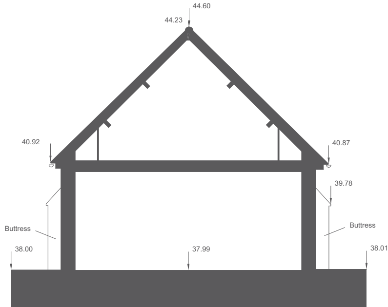
02 - PROPOSED SECTION 2
