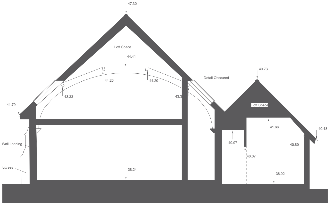
01 - PROPOSED SECTION 1
