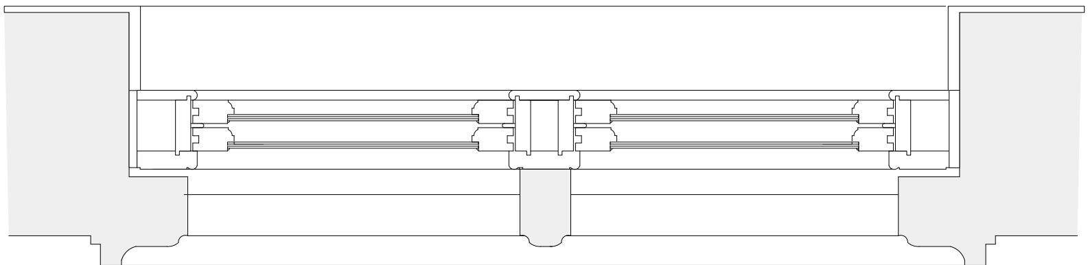
Sash Plan Detail
