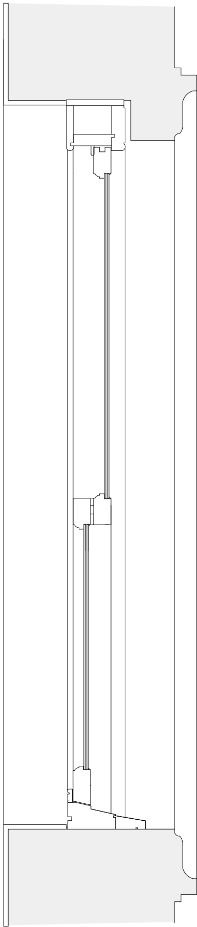
Sash Section Detail
