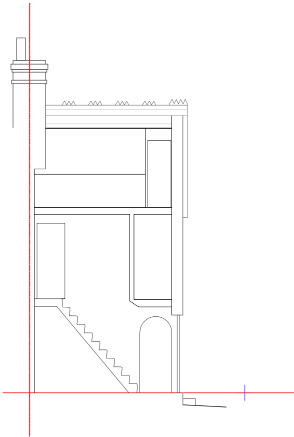
SIDE ELEVATION BB
