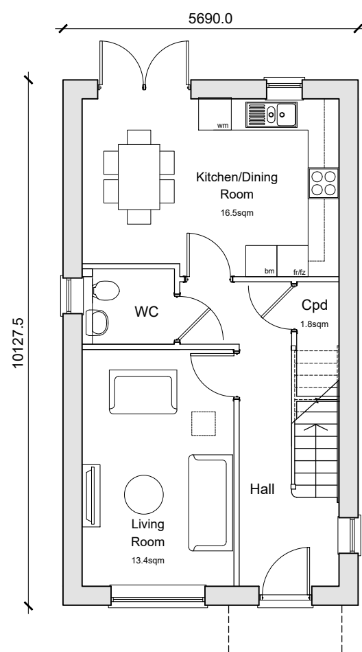
Ground Floor Plan HT31 3-Bedroom 5-Person House 65.0sqm (1,102sqft) GFA, 10 rooms A minimum of 2.5 sqm storage provided in accordance with NDIS requirements.
