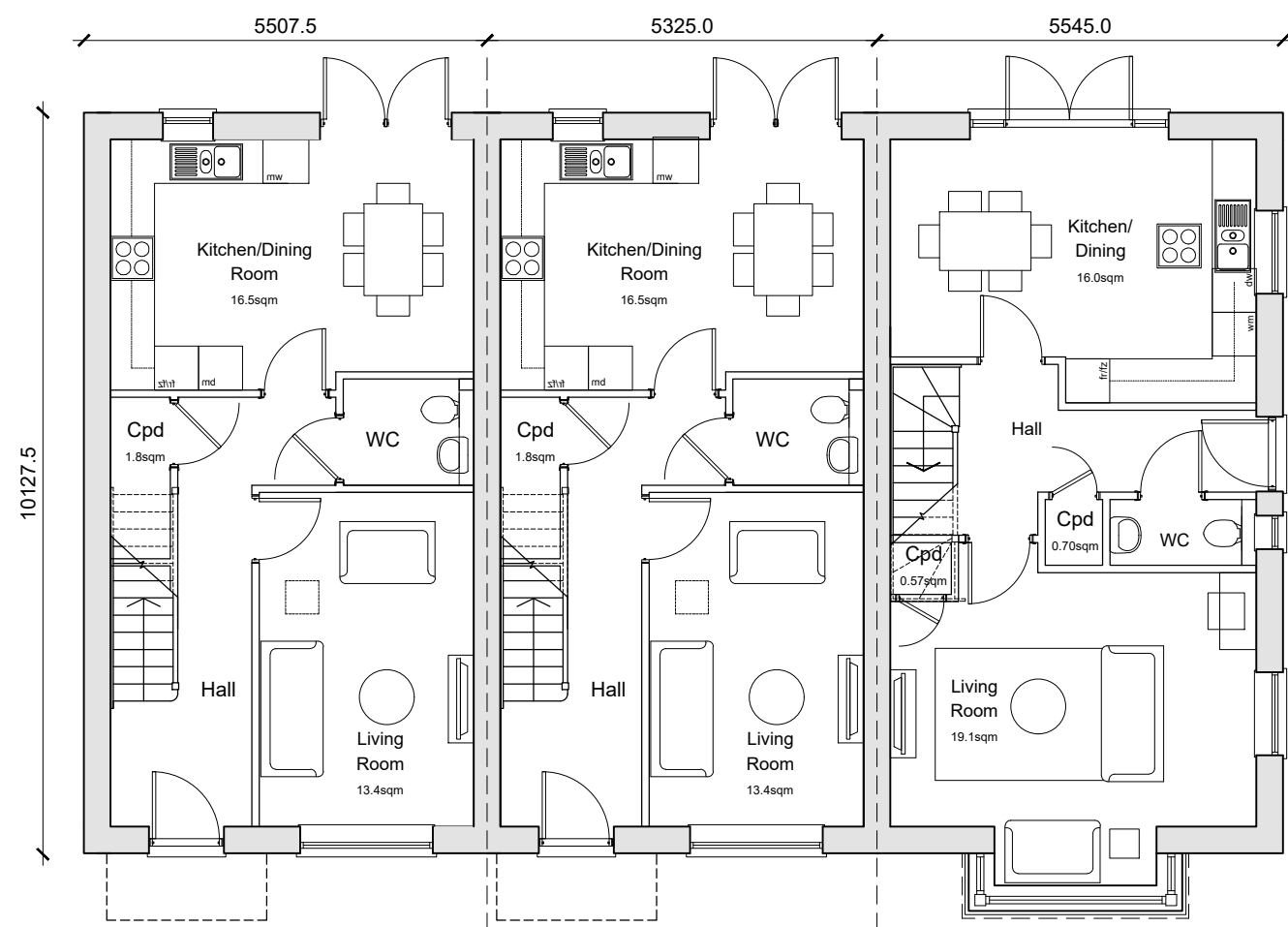
Ground Floor Plan HT31 3-Bedroom 5-Person House 33.4sqm (1100sqft GFA, 30.4sqm net) A minimum of 2.5 sqm storage provided in accordance with NDIS requirements.
