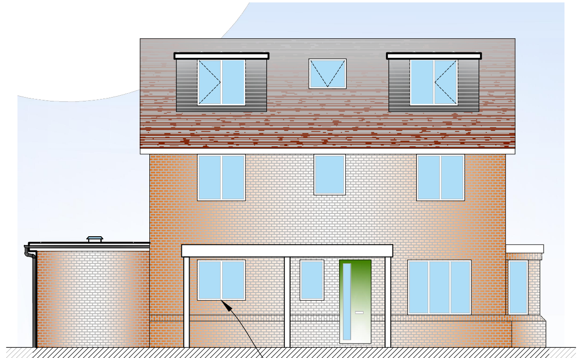
03 Side Elevation - As Proposed 3001 1:100 (at A3)
