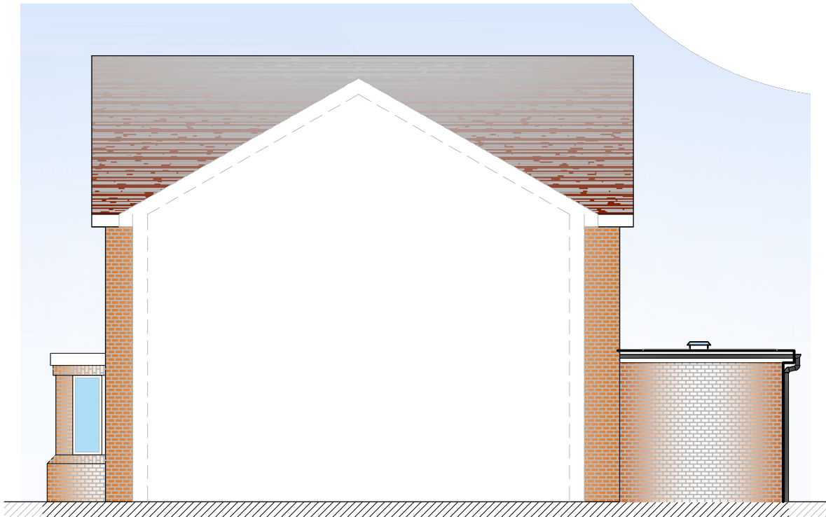
01 Side Elevation - As Proposed 3001 1:100 (at A3)
