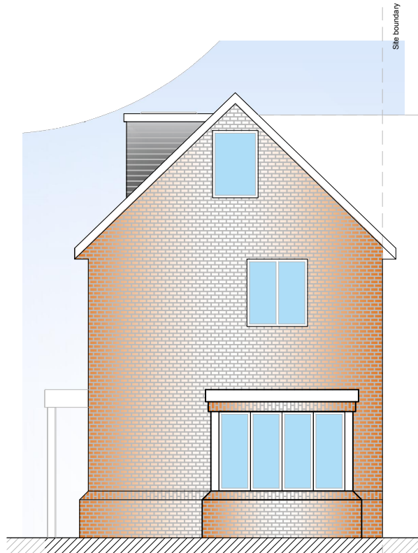
02 Rear Elevation - As Proposed 3001 1:100 (at A3)
