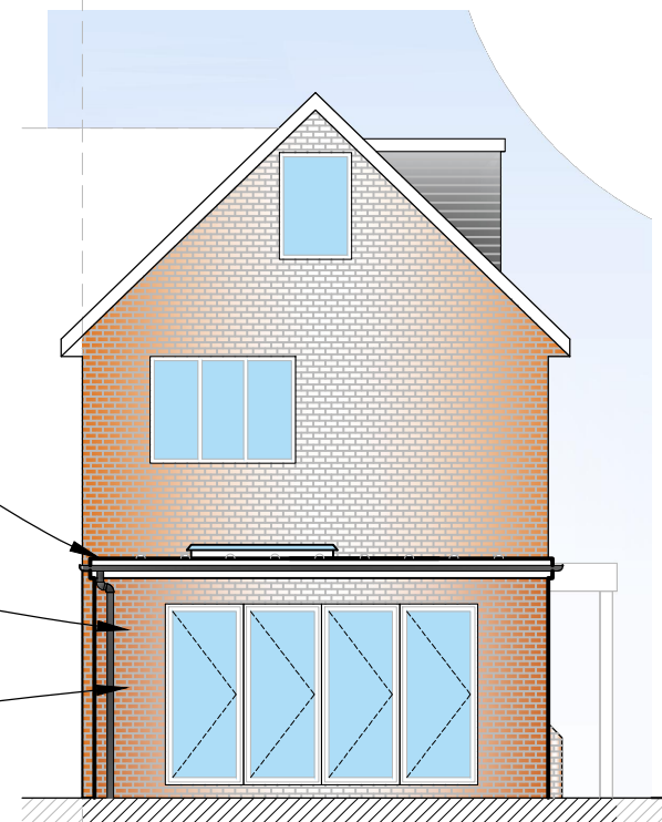
03 Side Elevation - As Proposed 3001 1:100 (at A3)
