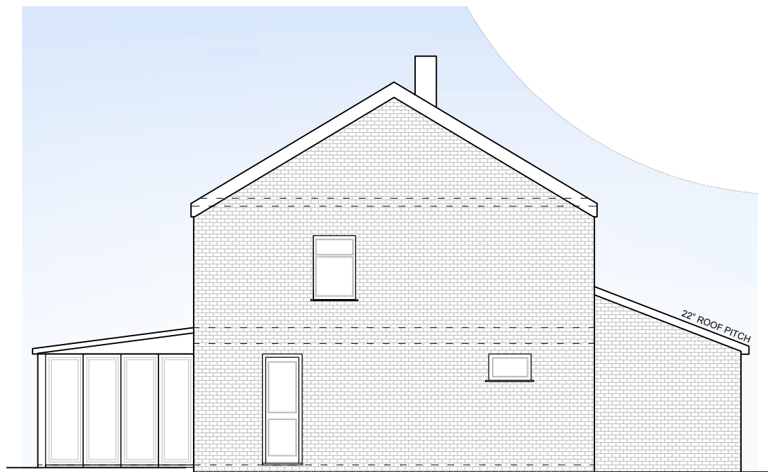
03 North Elevation - Proposed 3001 1:100 (at A3)
