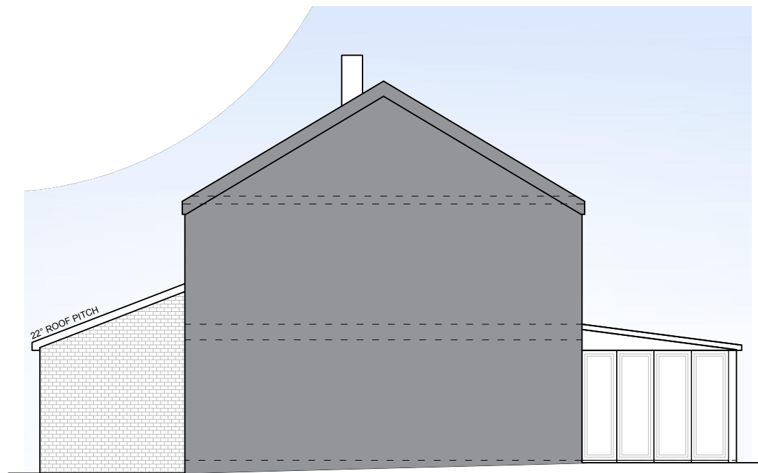
02 South Elevation - Proposed 3001 1:100 (at A3)
