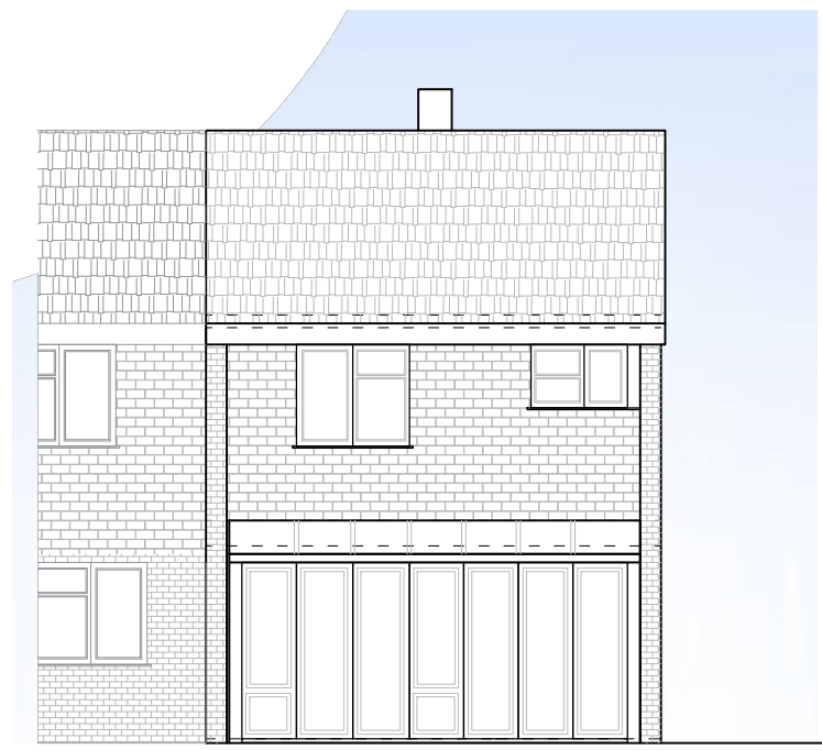
04 East Elevation - Proposed 3001 1:100 (at A3)
