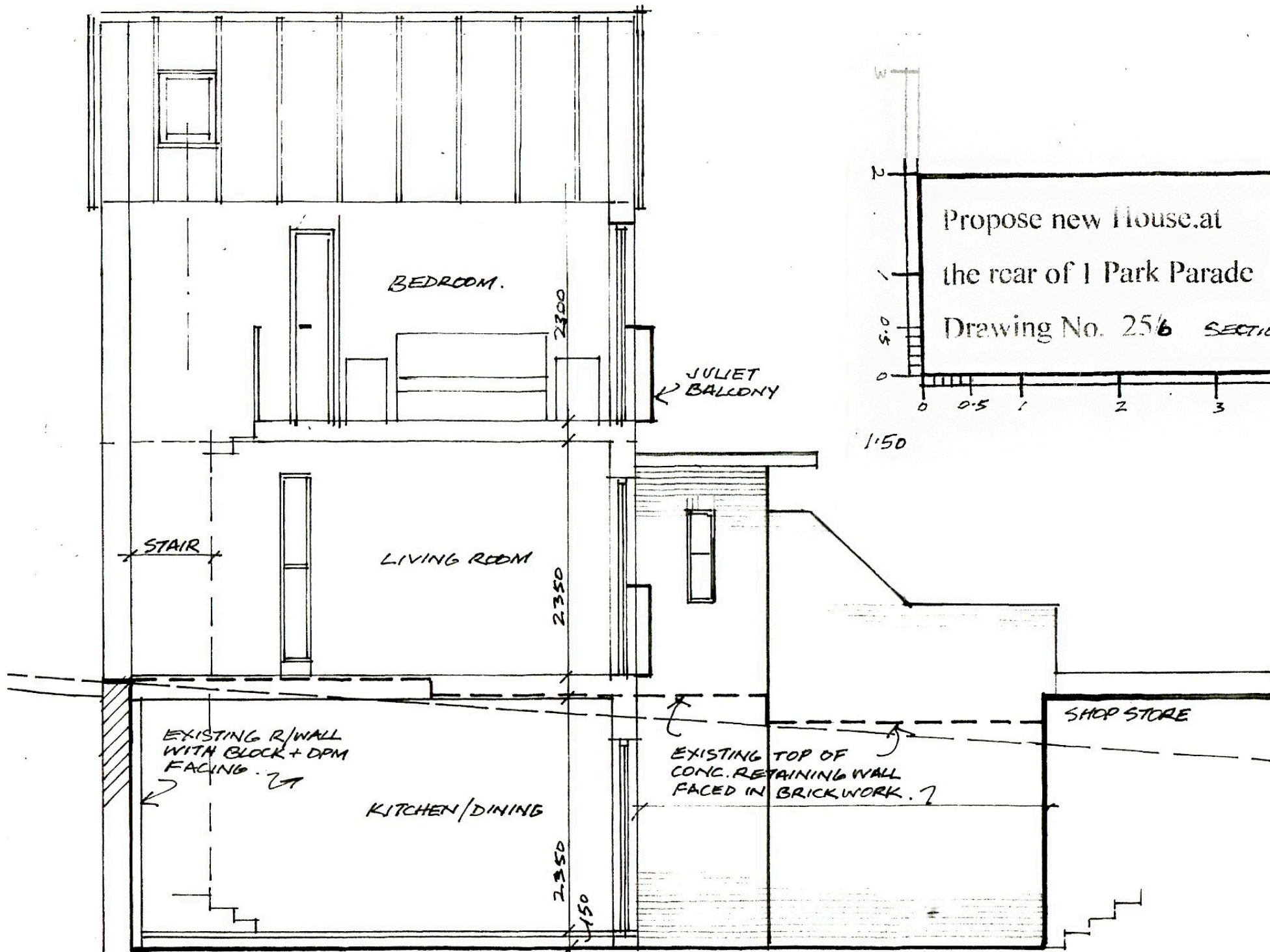
SECTION AA
