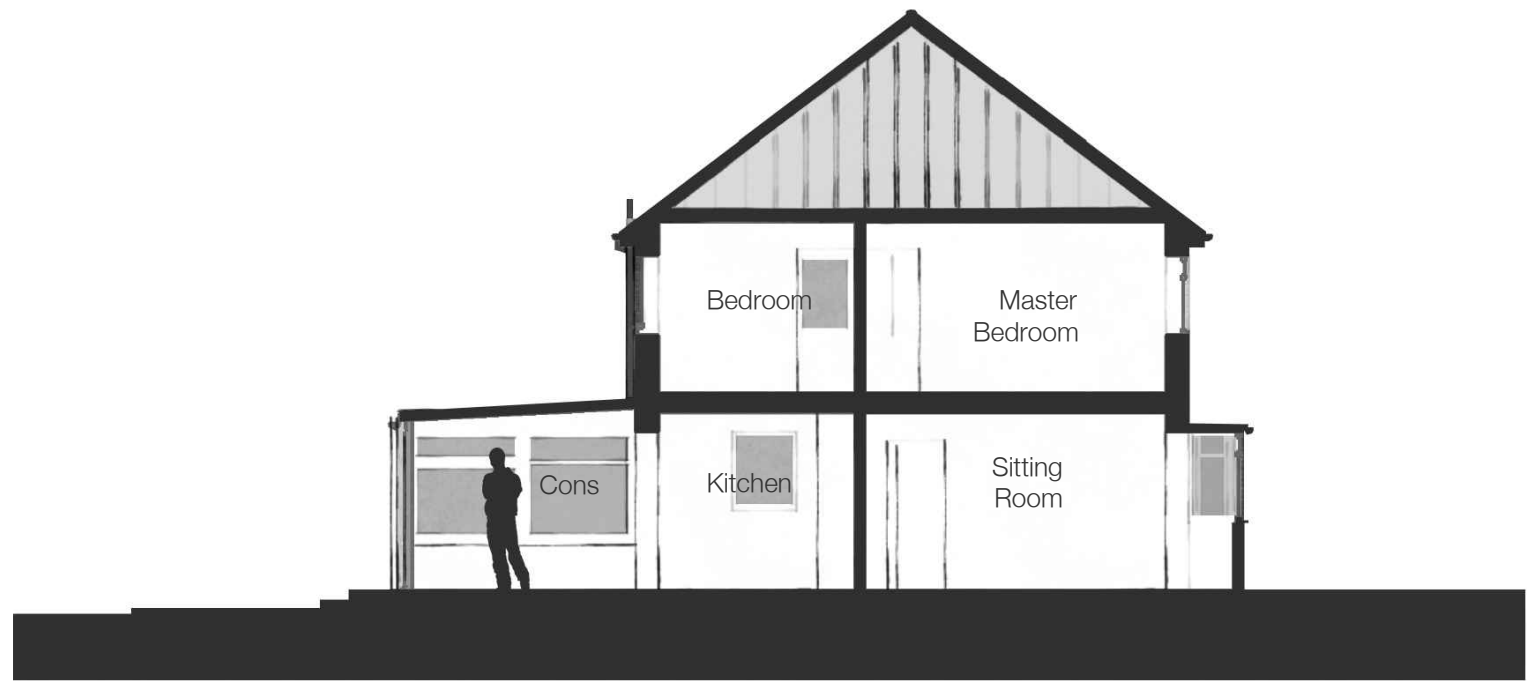
Existing Section 1
