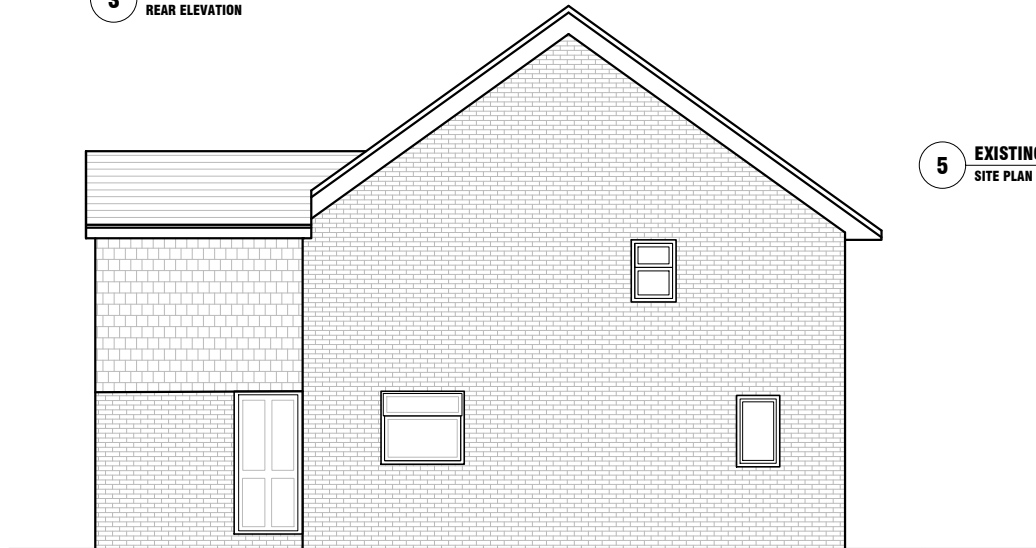
4 EXISTING SIDE ELEVATION 1:100
