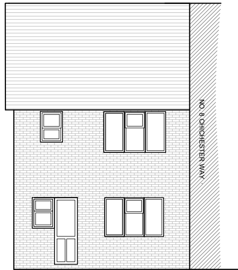
3 EXISTING REAR ELEVATION 1:100
