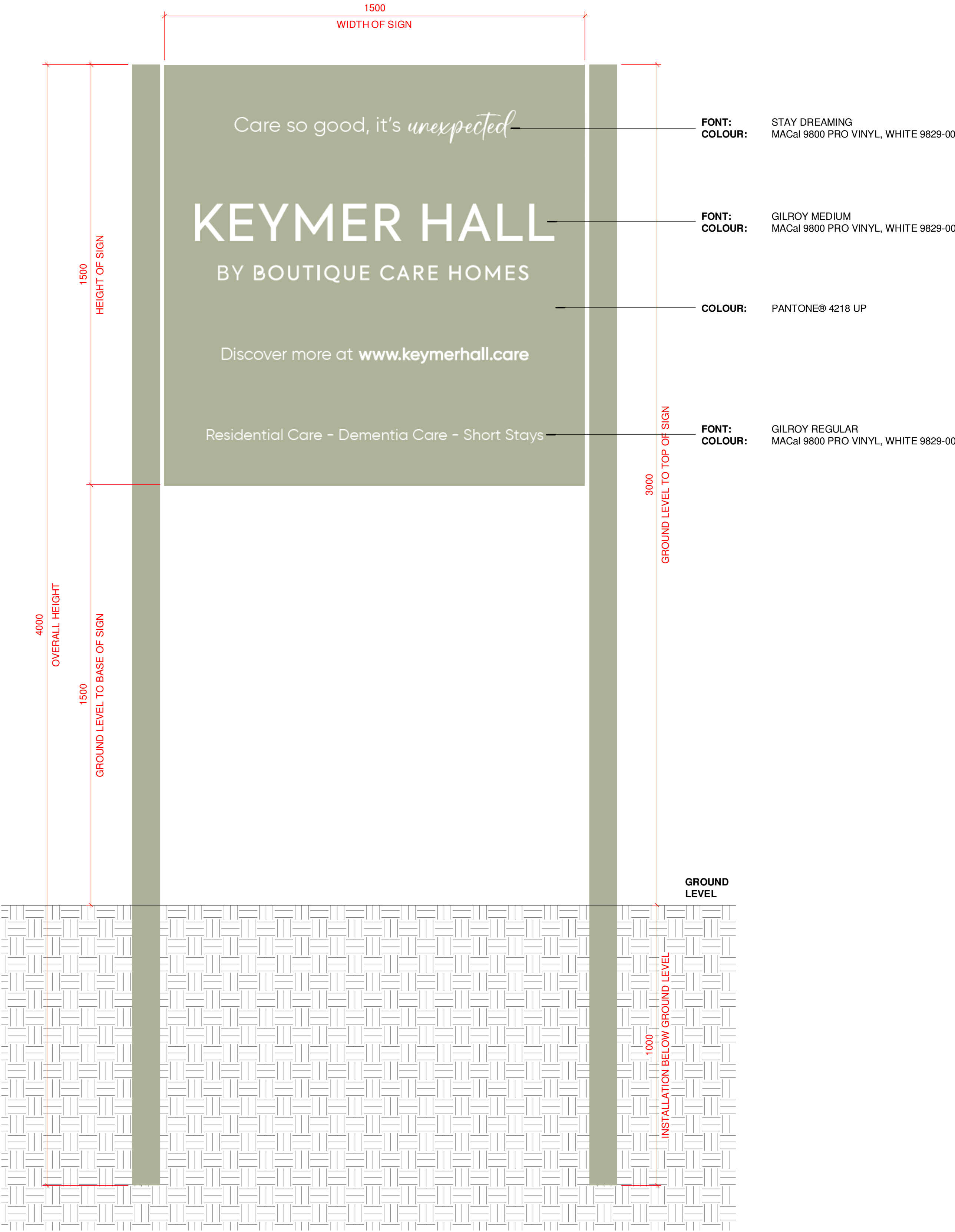
Proposed Signage - Elevation. 1 : 10
