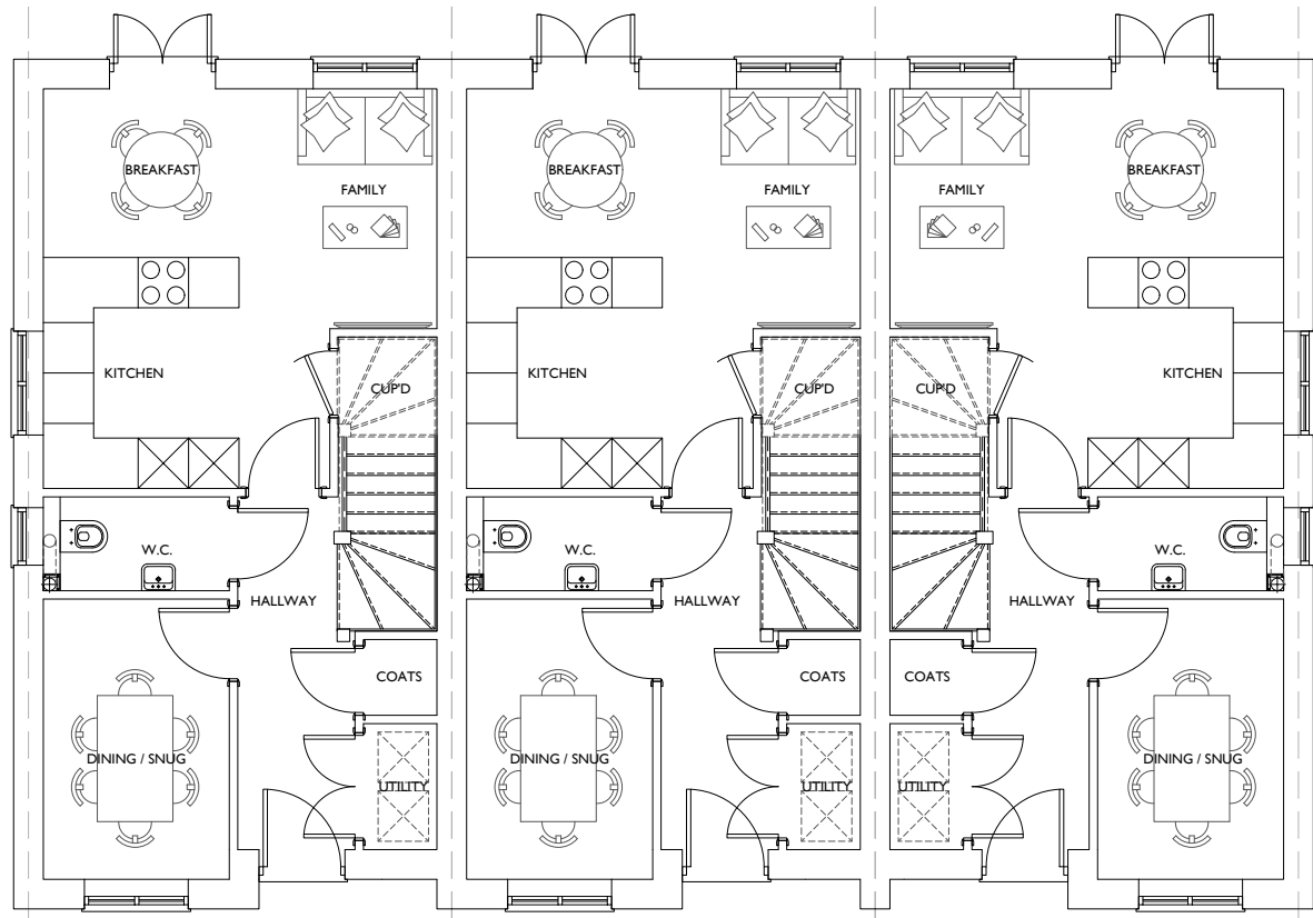
GROUND FLOOR PLAN HOUSE TYPE D1 & E1 - 127.53 sqm
