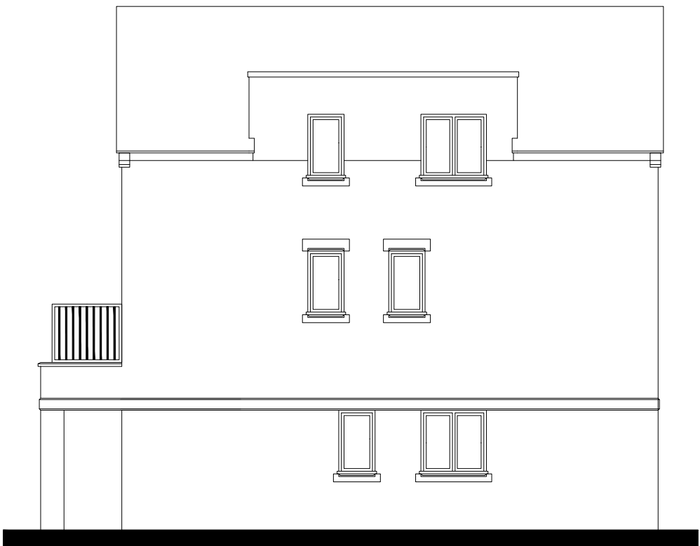
SIDE ELEVATIONS
