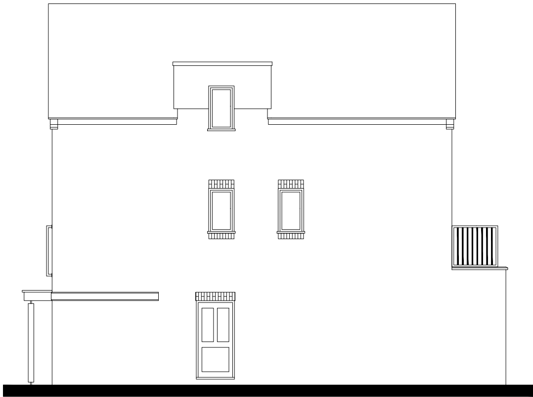
SIDE ELEVATIONS
