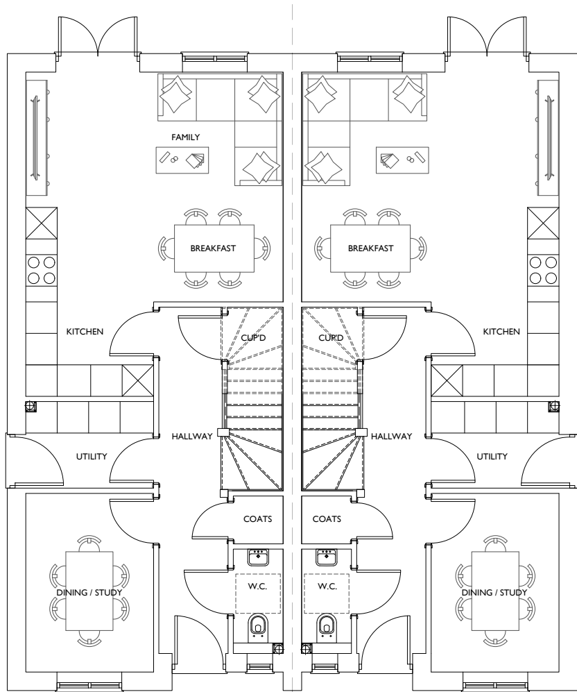
GROUND FLOOR PLAN HOUSE TYPE M1 - 149.25 sqm
