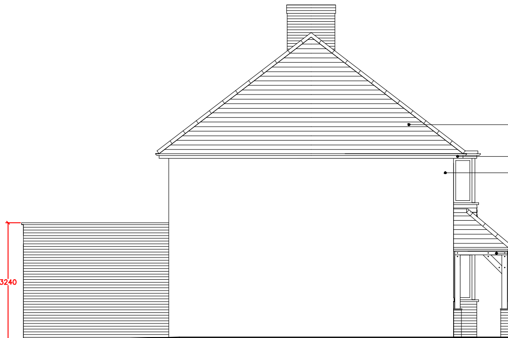
Side Elevation(North East Facing) (Scale 1:100)
