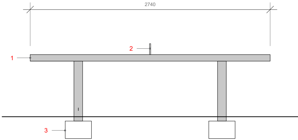
Front View 1:50
