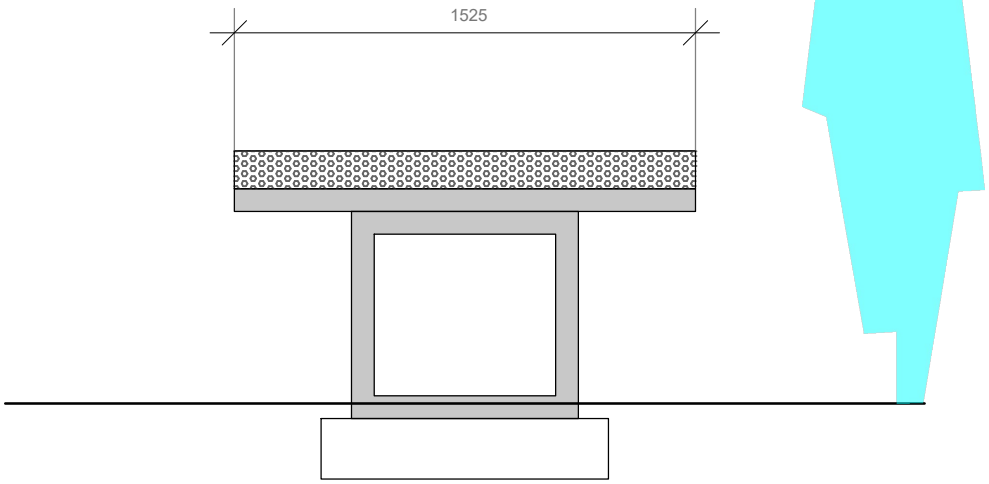
Side View 1:50
