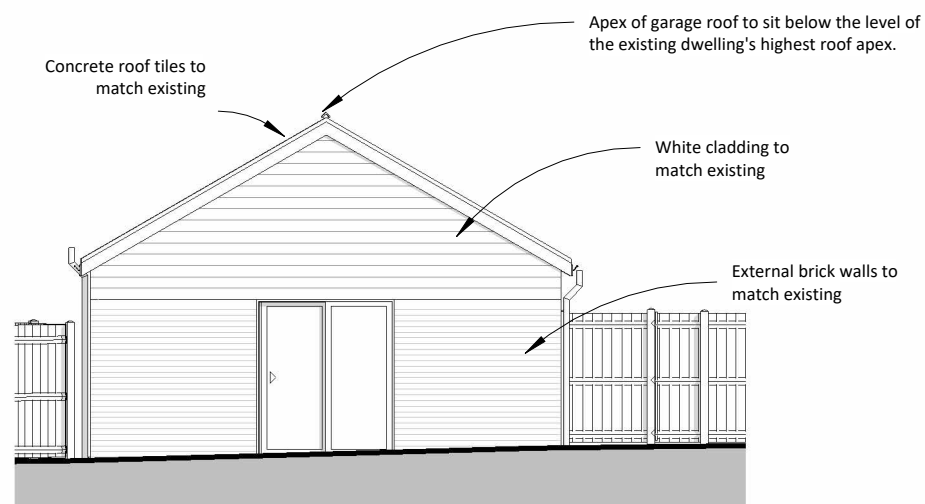
2 Garage Rear (West) Elevation 1 : 100
