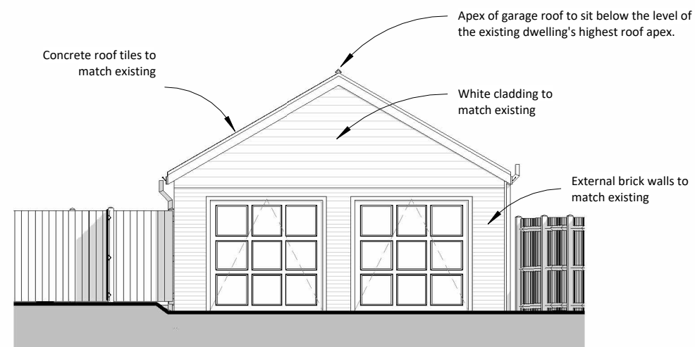
1 Garage Front (East) Elevation 1 : 100
