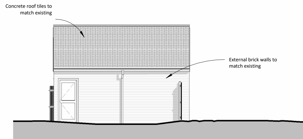
4 Garage Side (South) Elevation 1 : 100
