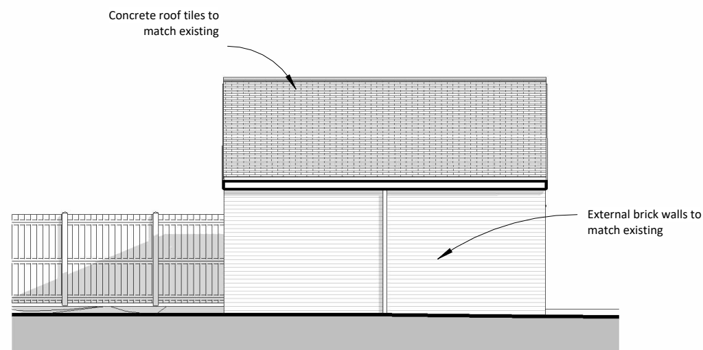
3 Garage Side (North) Elevation 1 : 100
