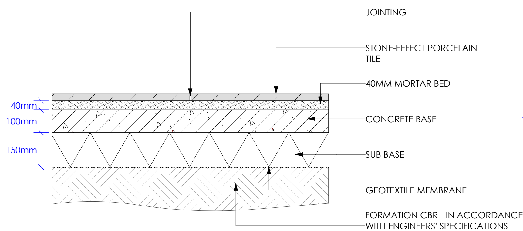
1 TYPICAL SECTION - STONE-EFFECT PORCELAIN TILE PAVING Scale: 1:10
