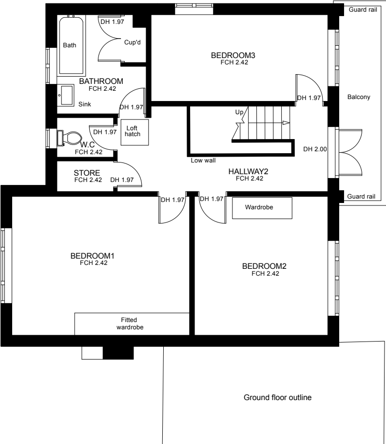
FIRST FLOOR
