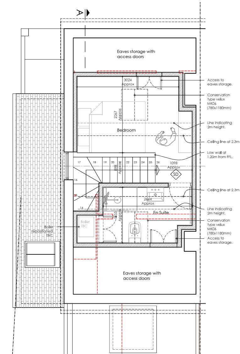
Proposed Second Floor Plan Scale 1/50@A3
