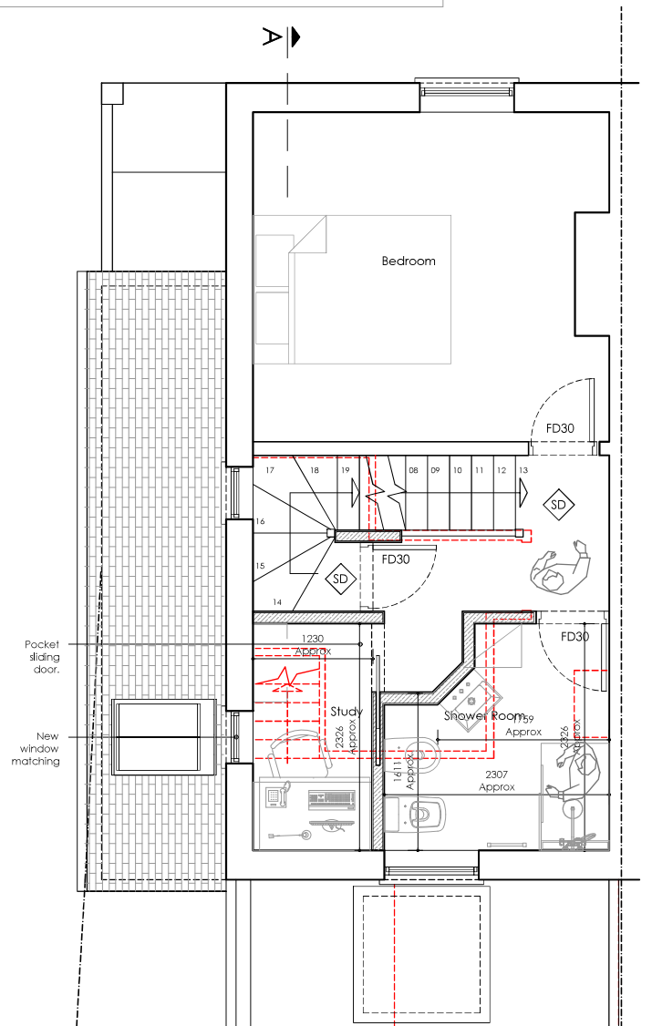
Proposed First Floor Plan Scale 1/50@A3
