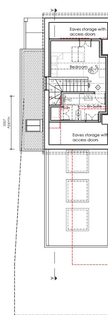
Proposed Second Floor Plan Scale 1/100@A3
