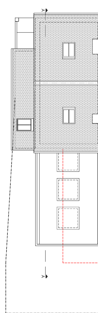
Proposed Roof Plan Scale 1/100@A3
