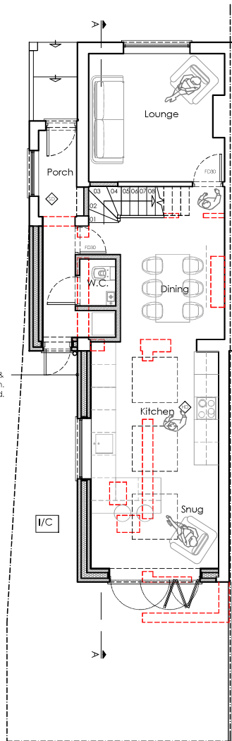
Proposed Ground Floor Plan Scale 1/100@A3
