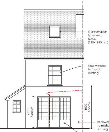
Proposed Rear Elevation Option A Scale 1/100@A3
