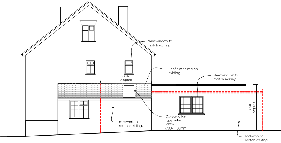
Proposed RHS Elevation Option A Scale 1/100@A3
