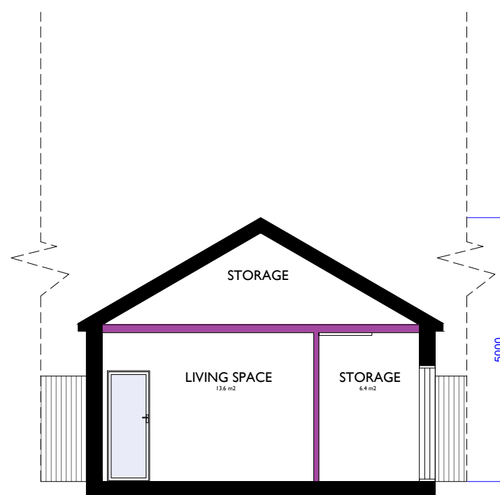
Proposed A-A Section
