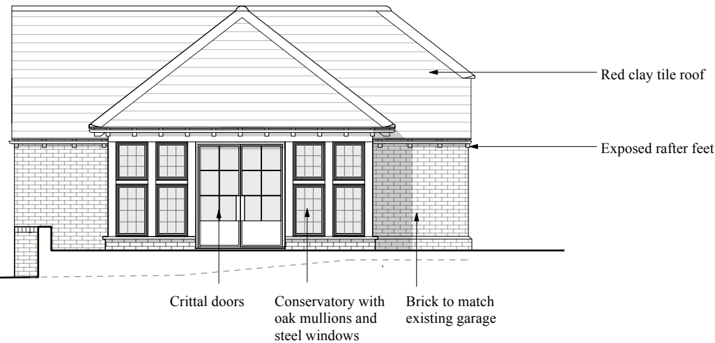
East Elevation
