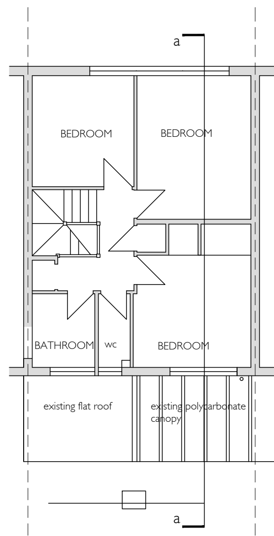
existing ground and first floor plans 1:100
