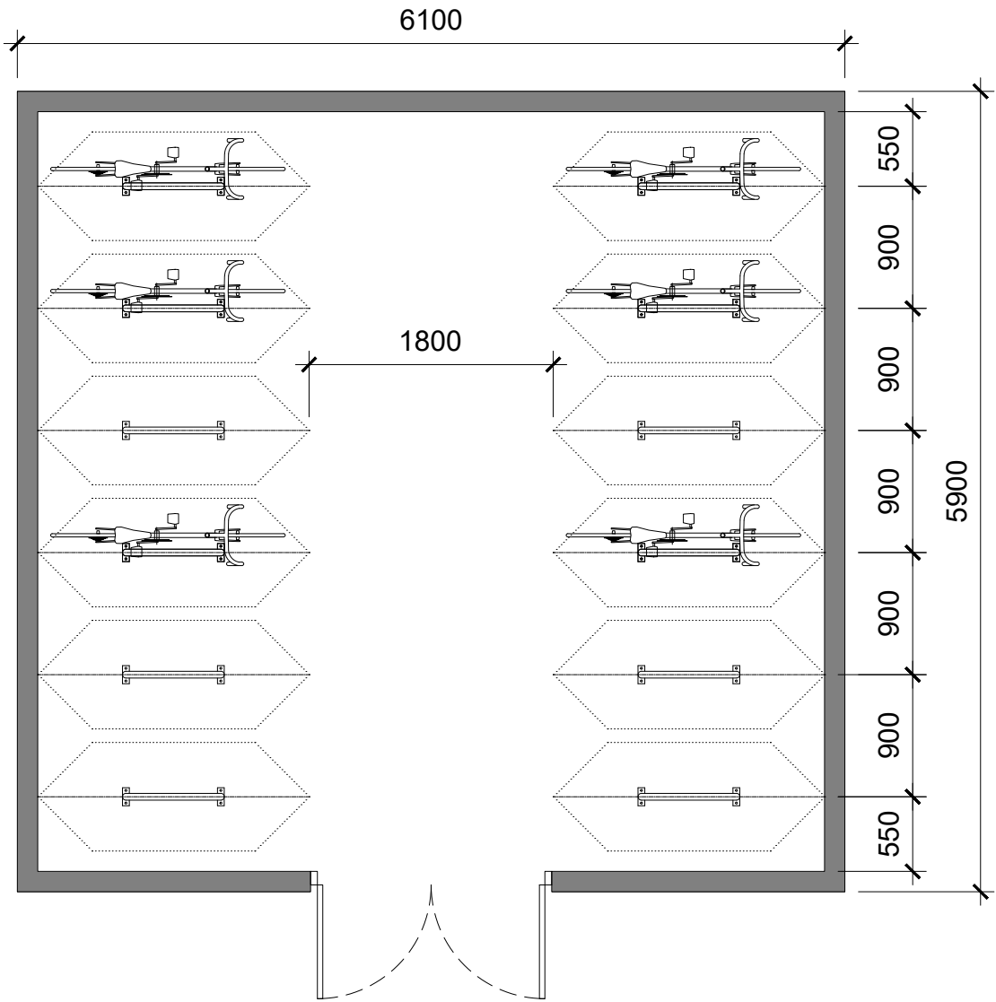
Cycle Store Plan
