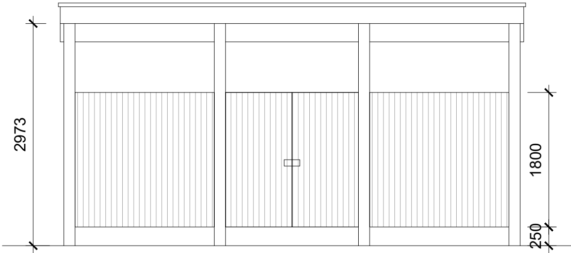
Front Elevation
