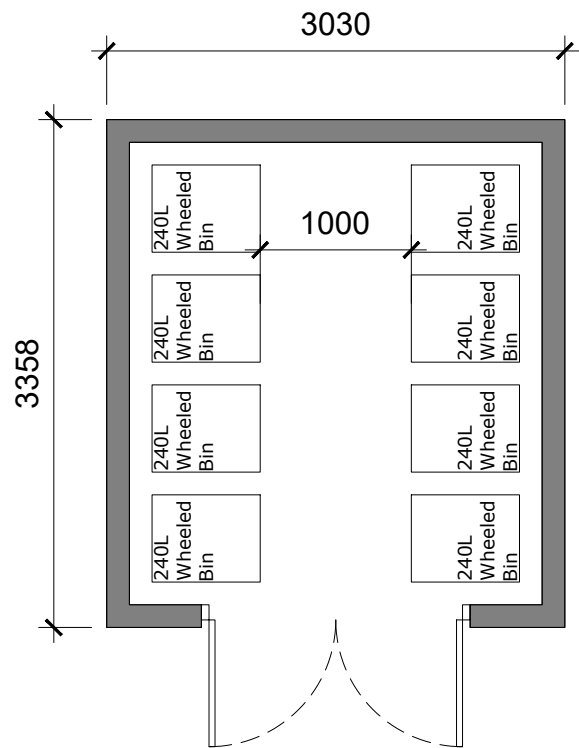
Bin Store Plan
