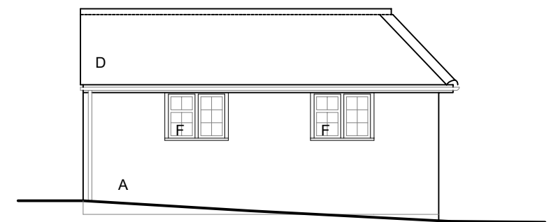
G - Existing South-West Elevation
