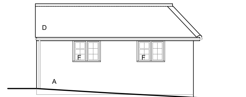
I - Existing North-West Elevation
