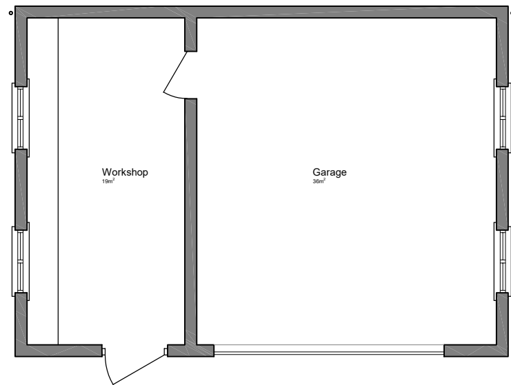
1- Proposed Ground Floor Plan (as existing)
