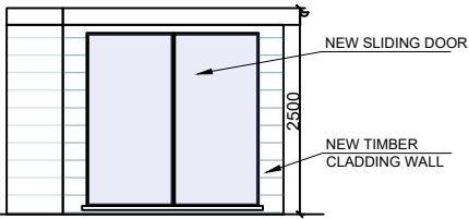
Proposed South Elevation
