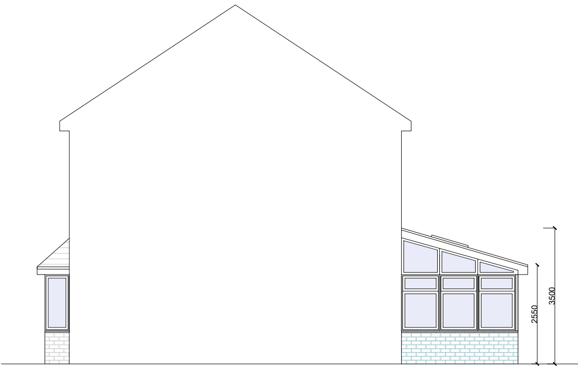
Proposed West Elevation (Between Garage and Conservatory)
