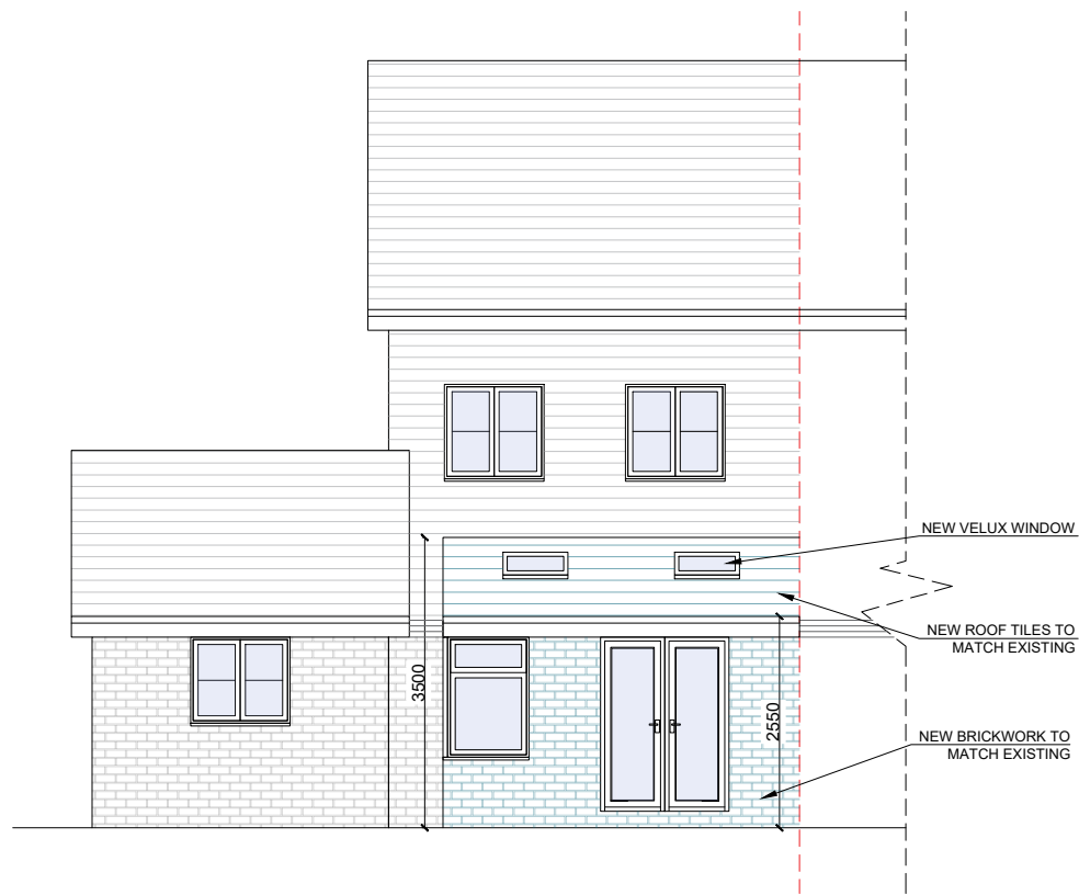
Proposed South Elevation
