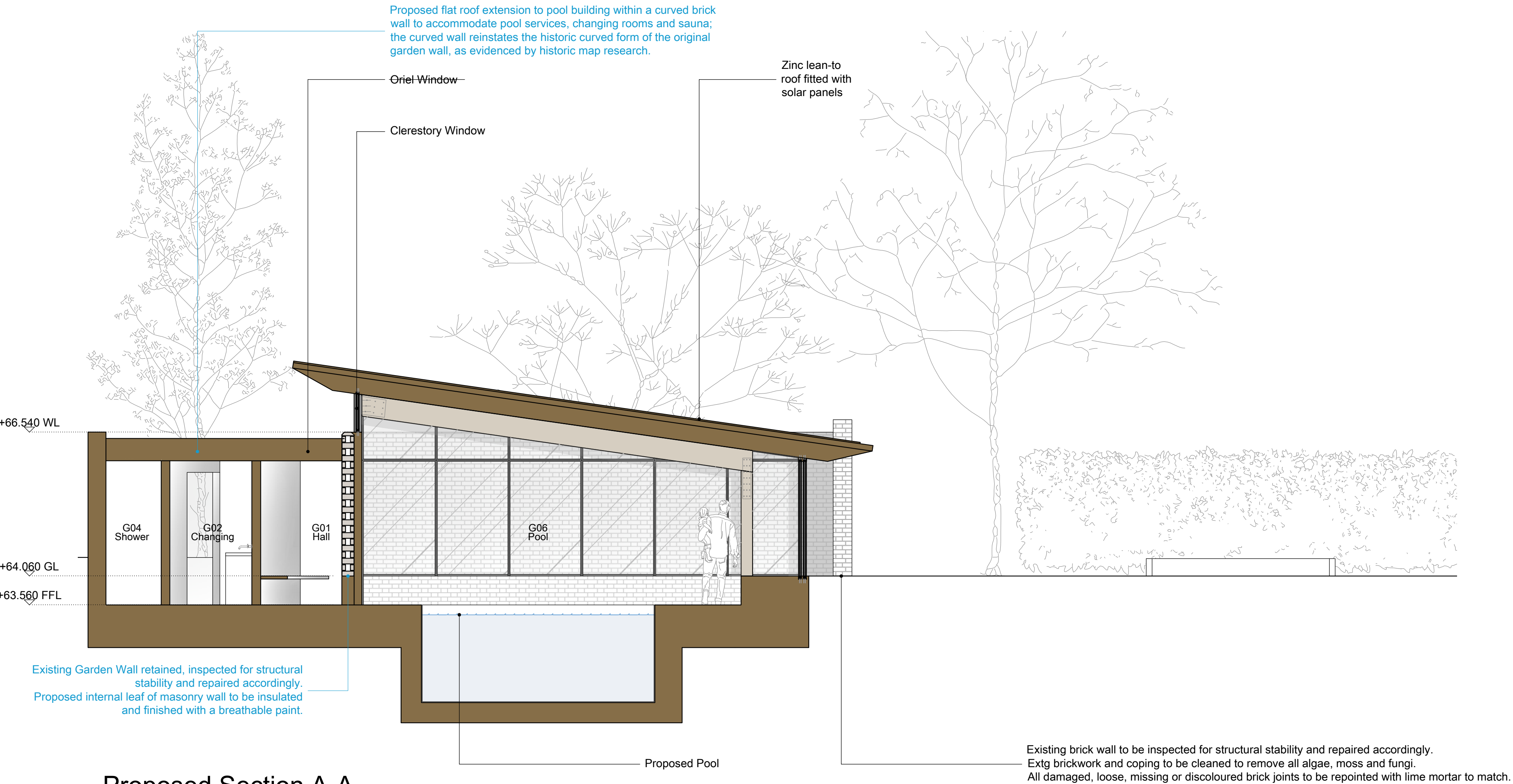
01 Proposed Section A-A 1:50 @ A1 ; 1:100 @ A3
