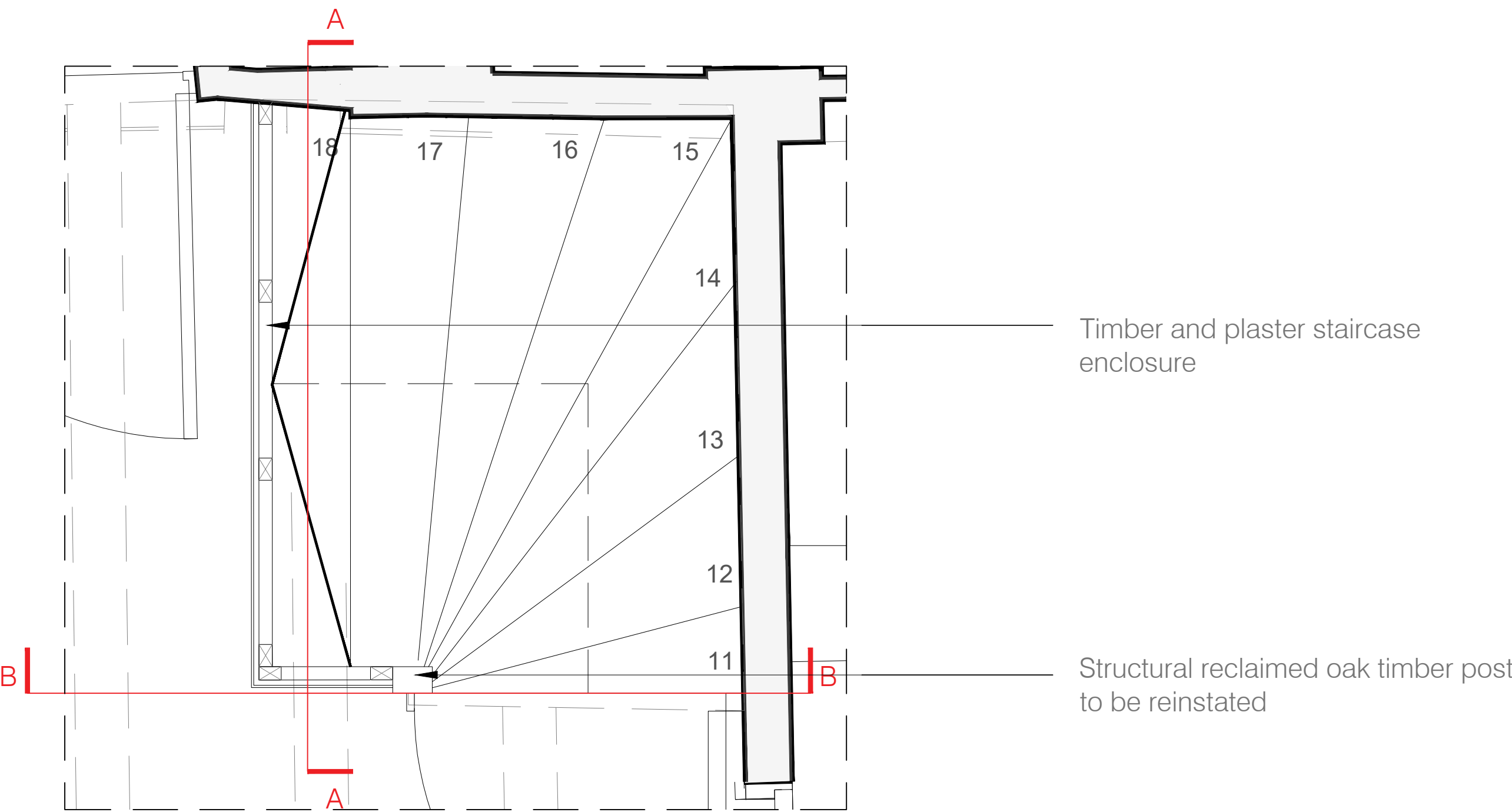
First Floor Staircase Plan, Scale 1:10@A1, 1:20@A3
