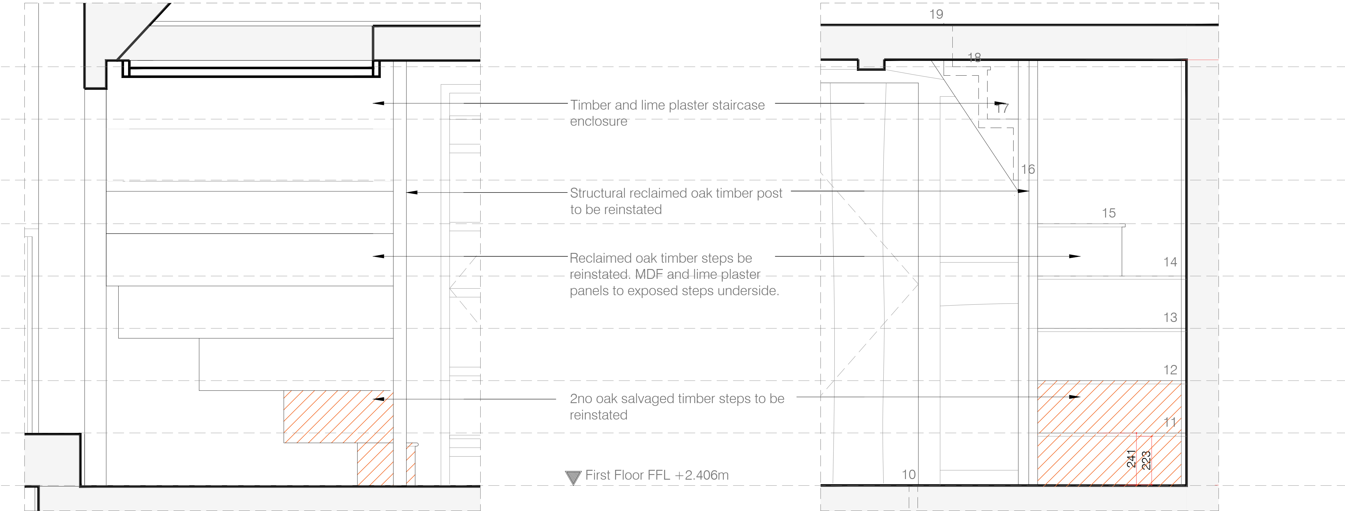
First Floor Staircase Section AA Scale 1:10@A1, 1:20@A3
