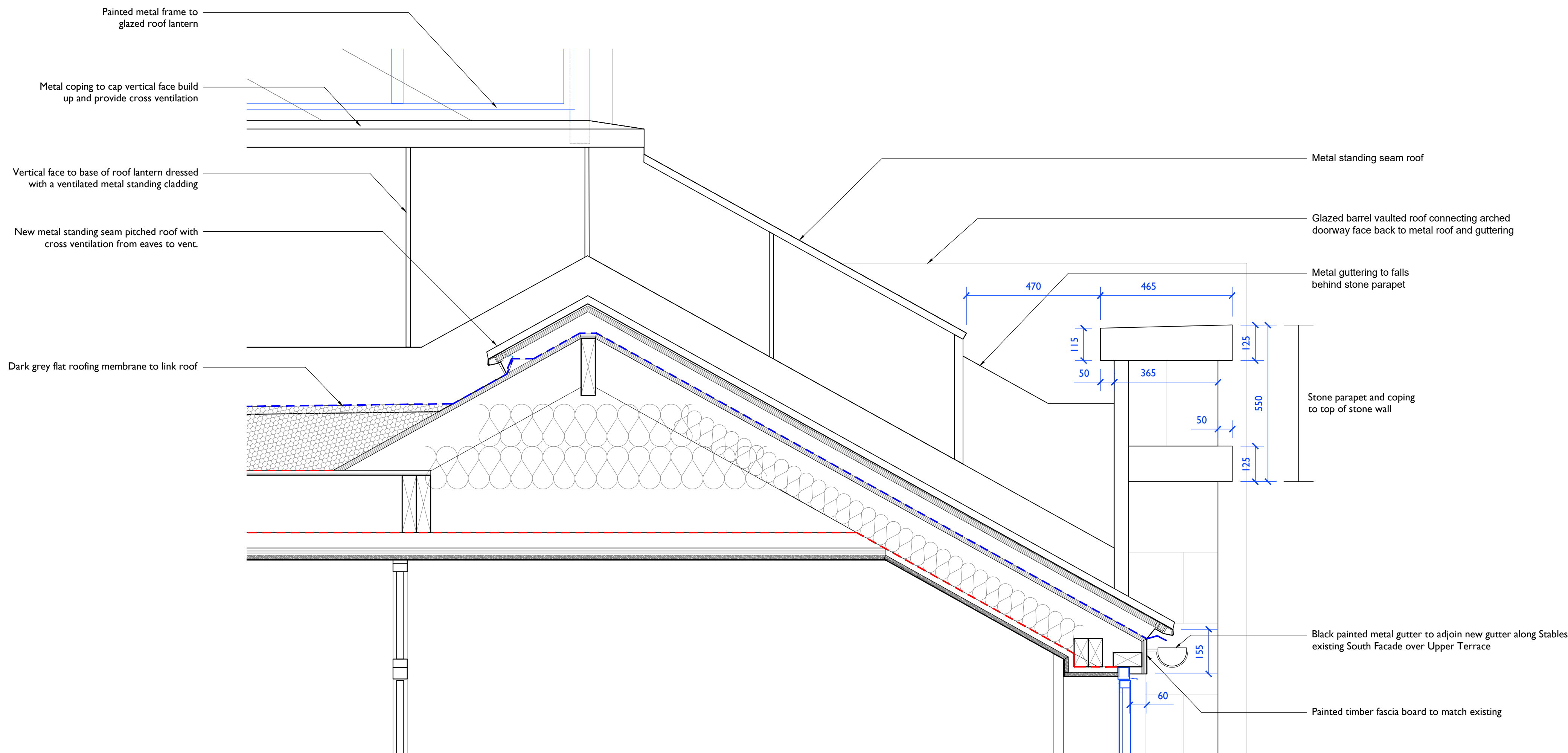
I Proposed West Glasshouse Entrance - Detail Section to Eaves 5107 I:10 @ A1, I:20 @ A3
